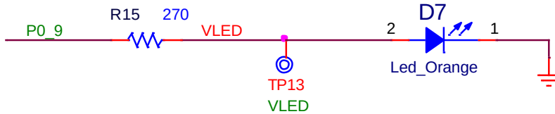
Figure 20. General-purpose LED
