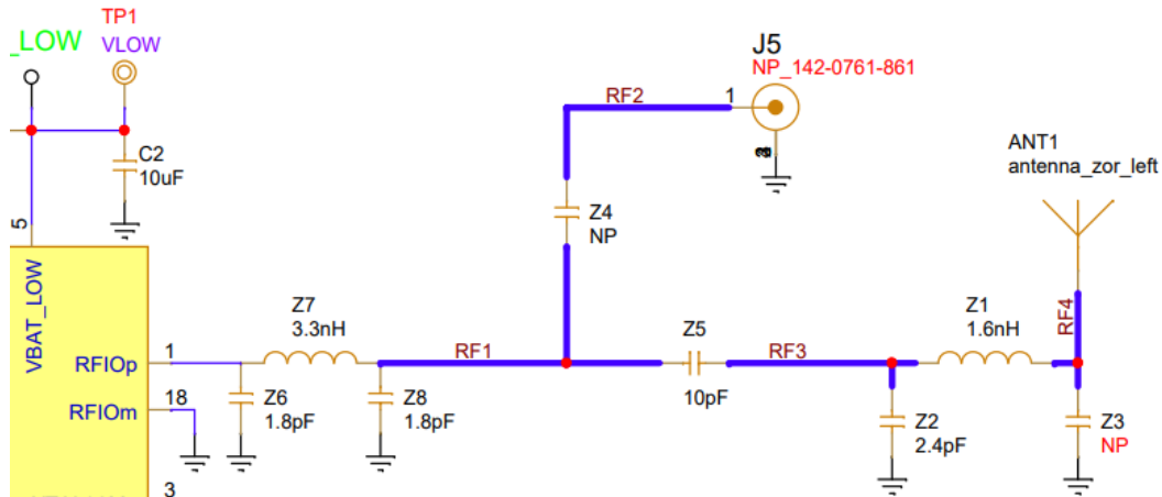
Figure 9. RF section
