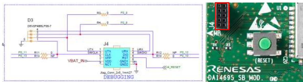
Figure 10: CIB (JTAG/UART interface) connector (J4)
