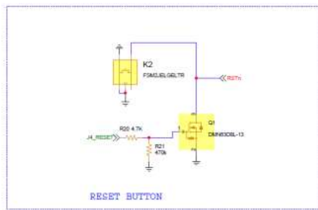
Figure 8: Reset button on DA14695 SmartBond module DB
