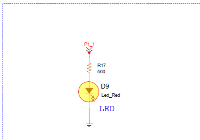
Figure 9: General purpose LED on DA14695 SmartBond module DB
