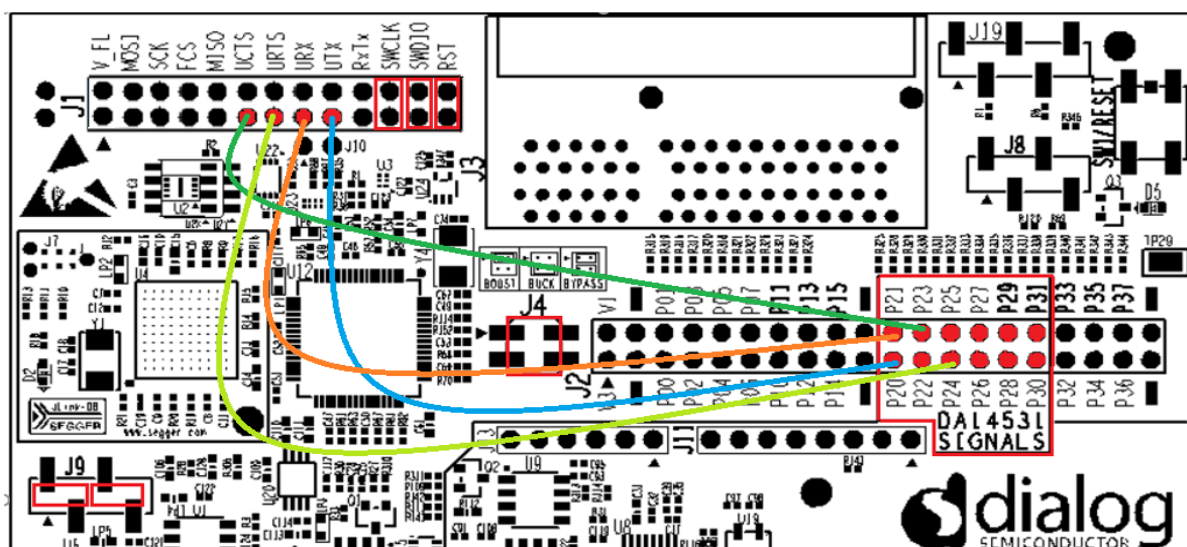
Figure 26: Full UART (4-wire) Connectivity
