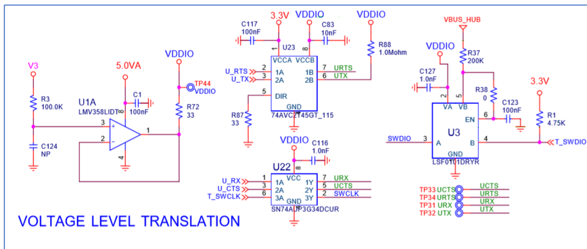
Figure 15: Voltage Translator Circuitry of DA14531 PRO-MB
