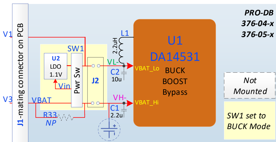
Figure 6: DA14531 PRO-DB Power Section
