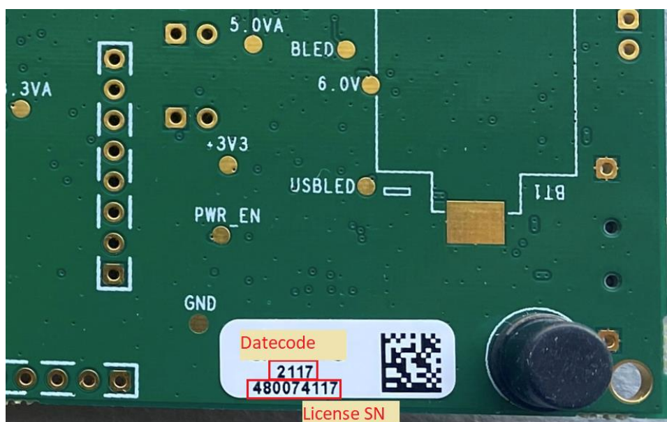
Figure 78: Label on DA14531 PRO-MB PCBA
