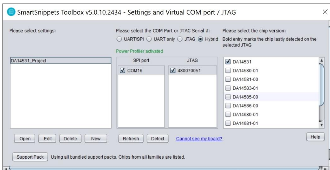
Figure 39: Hybrid Configuration
