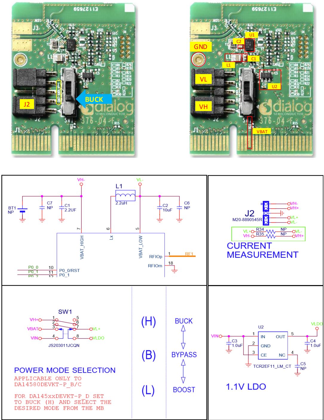
Figure 7: Power Section of DA14531 PRO-DB
