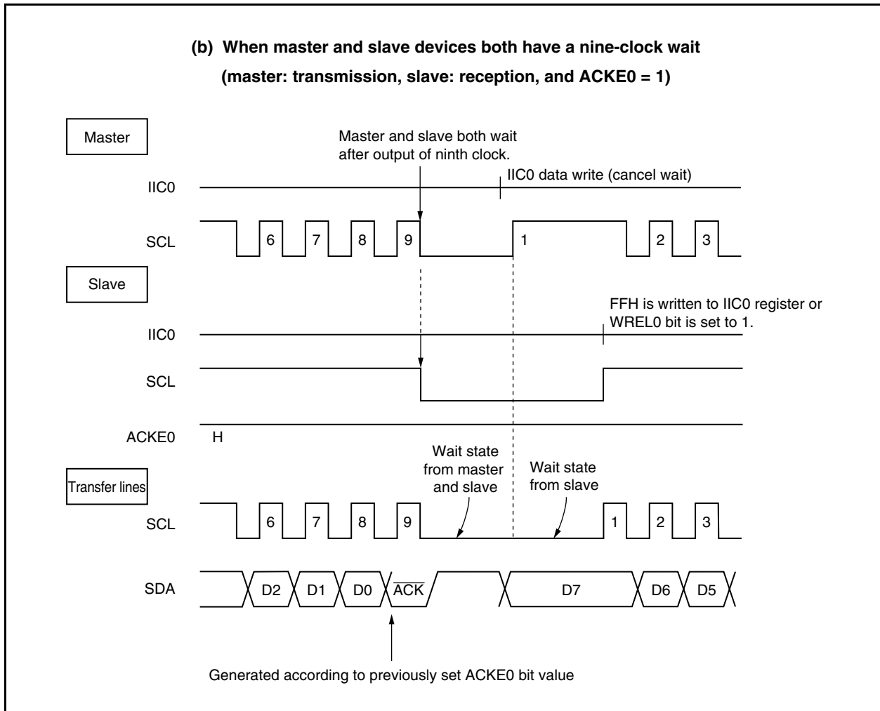
Figure 17-11. Wait State (2/2)
