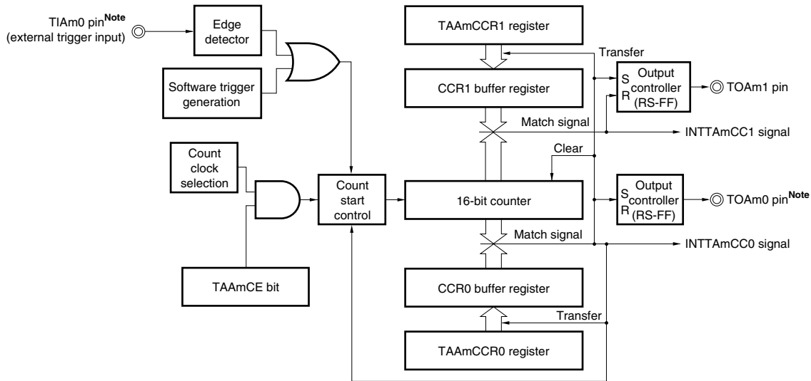
Figure 6-28. Configuration in One-Shot Pulse Output Mode
