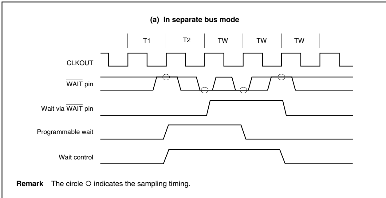
Figure 18-1. Example of Inserting Wait States (1/2)
