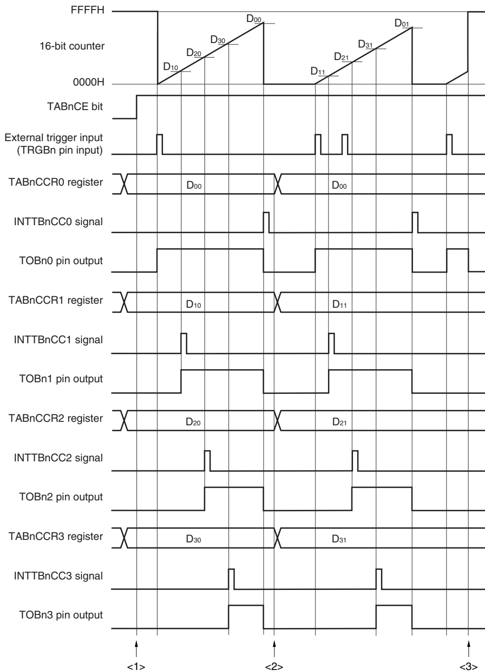
Figure 7-27. Software Processing Flow in One-Shot Pulse Output Mode (1/2)
