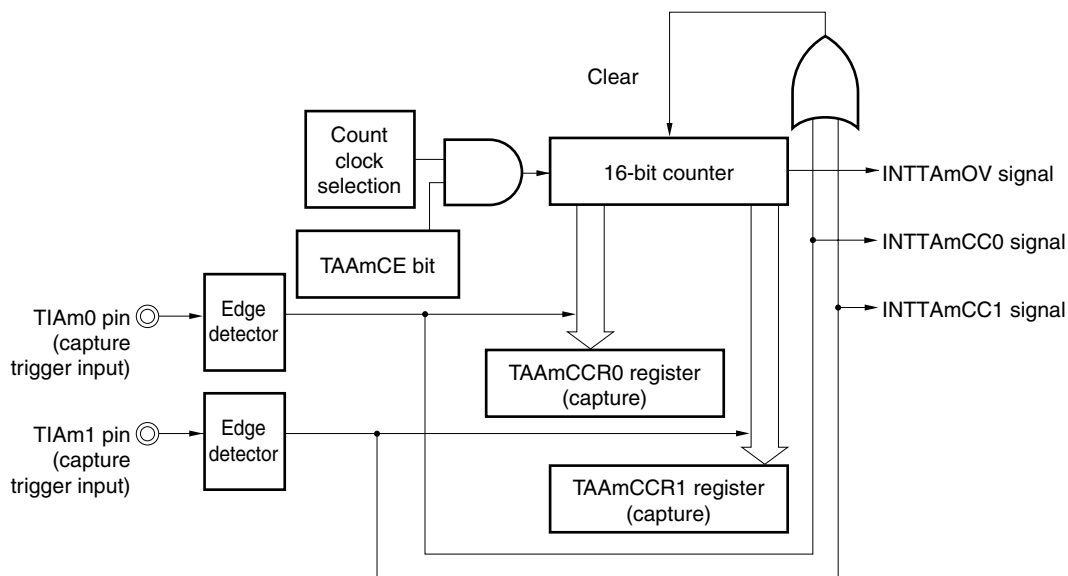
Figure 6-42. Configuration in Pulse Width Measurement Mode
