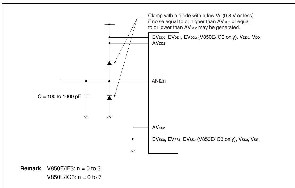
Figure 13-12. Processing of Analog Input Pin
