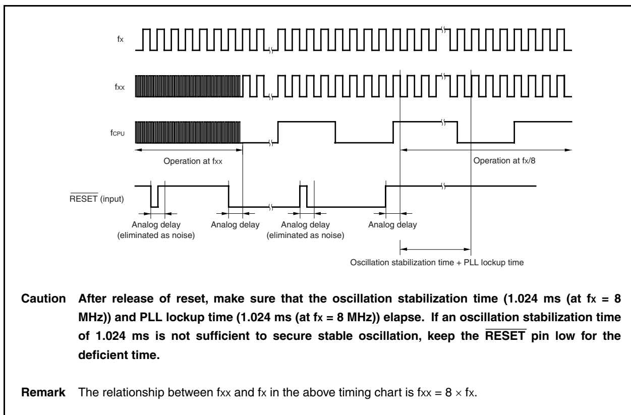
Figure 22-1. Reset Operation by \overline{\text{RESET}} Pin Input
