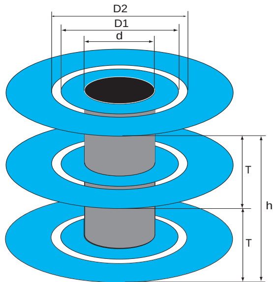
Figure 16: Via Construction
