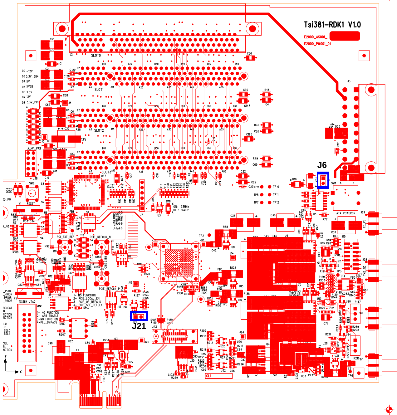
Figure 7: Shunt Jumper Locations
