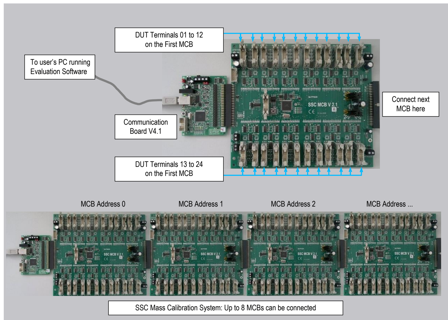
Figure 2. Modular Mass Calibration System (MCS)
