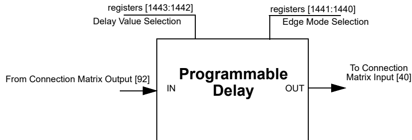
Figure 77: Programmable Delay
