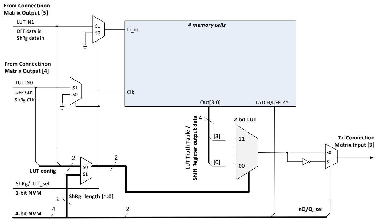
Figure 15: 2-bit LUT2 or DFF2 or Shift Register2
