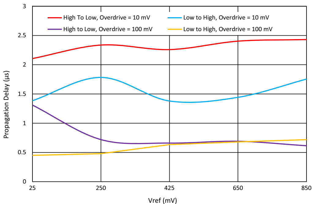
Figure 75: Typical Propagation Delay vs. Vref for ACMPxH at T = 25 °C, Gain = 1, Hysteresis = 0, V DD = 1.0 V to 1.65 V
