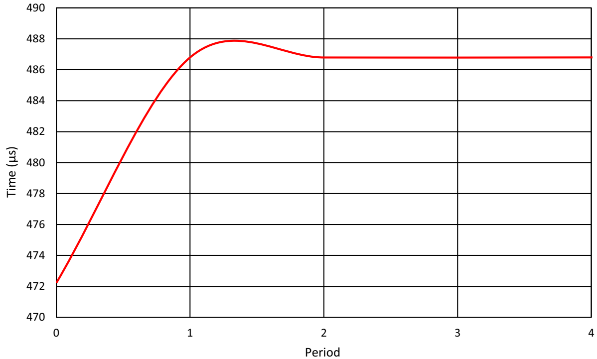
Figure 92: Oscillator0 Settling Time, V_{DD} = 1.2 V, T = 25 °C, OSC0 = 2.048 kHz
