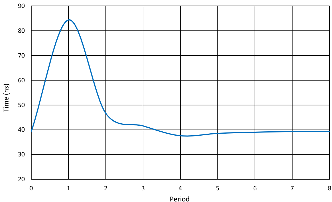
Figure 93: Oscillator1 Settling Time, V_{DD} = 1.2 V, T = 25 °C, OSC1 = 25 MHz (Normal Start)
