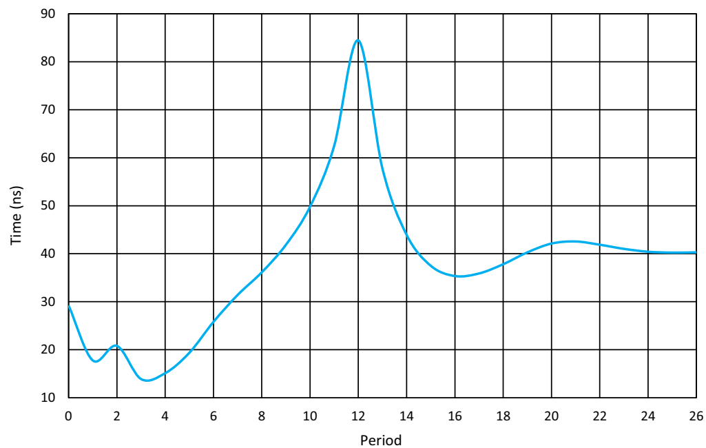
Figure 137: Oscillator1 Settling Time, V_{DD} = 3.3 \text{ V} , T = 25^\circ\text{C} , \text{OSC1} = 25 \text{ MHz} (Normal Start)
