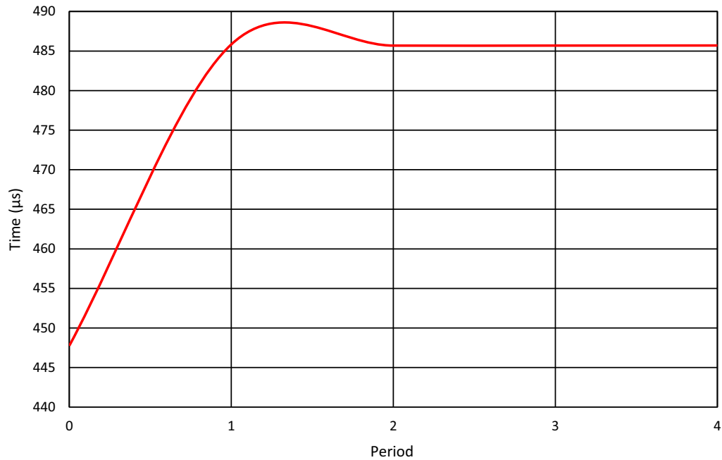
Figure 136: Oscillator0 Settling Time, V_{DD} = 3.3 \text{ V} , T = 25^\circ\text{C} , \text{OSC0} = 2 \text{ kHz}
