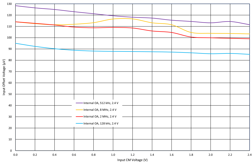
Figure 83: Internal OpAmp Input Offset Voltage vs. Input CM Voltage at T = 25^\circ\text{C} , V_{\text{DDA}} = 2.4\text{ V}
