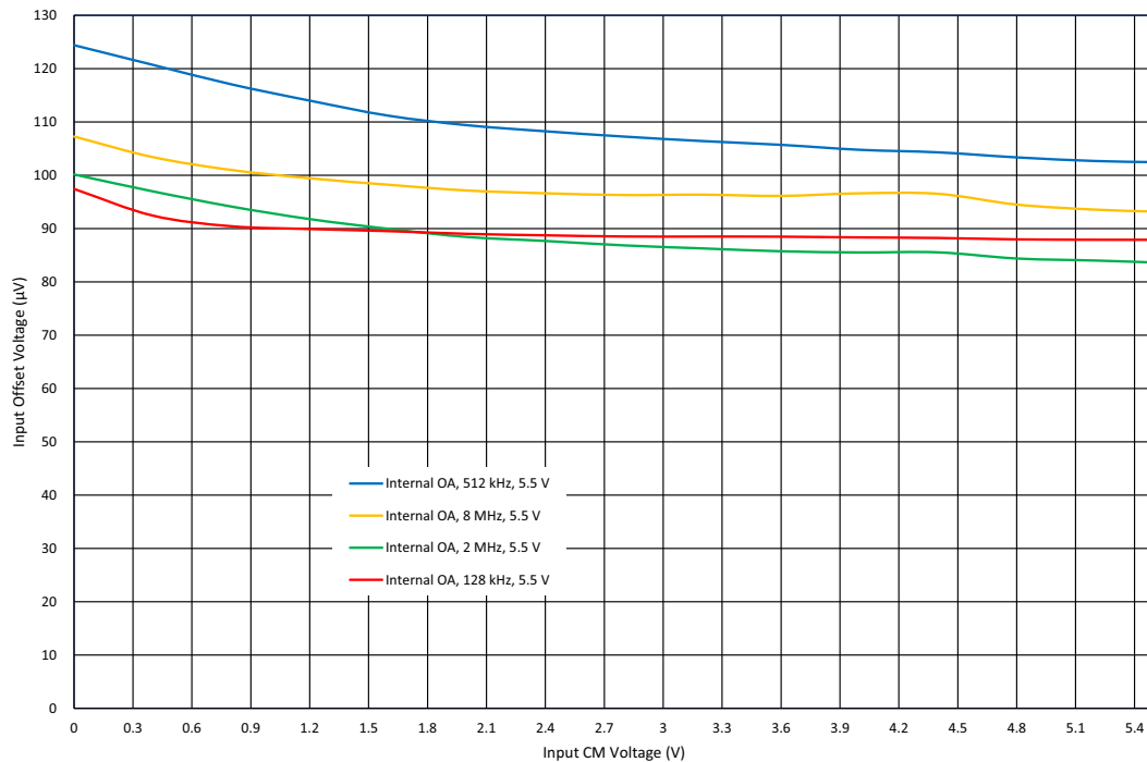
Figure 84: Internal OpAmp Input Offset Voltage vs. Input CM Voltage at T = 25\text{ }^{\circ}\text{C} , V_{DDA} = 5.5\text{ V}
