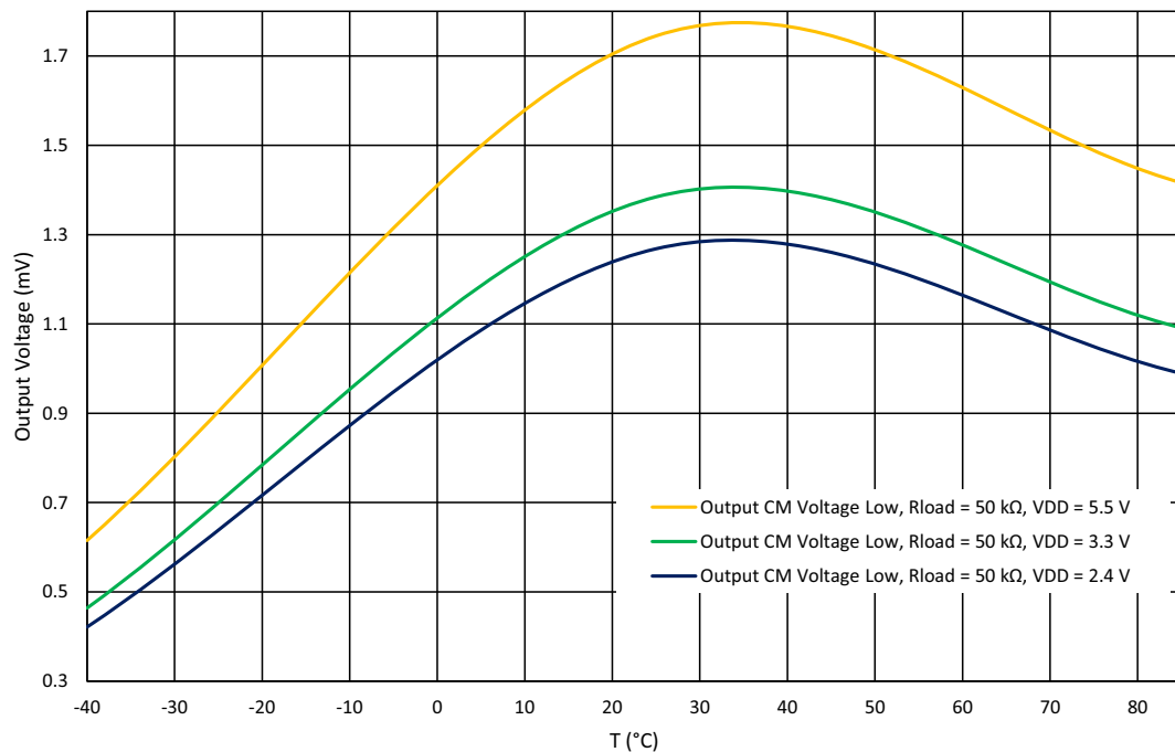
Figure 149: Output Voltage Low ( V_{\text{OUT}} - \text{GND} ) vs. Temperature at \text{BW} = 8\ \text{MHz} , R_{\text{LOAD}} = 50\ \text{k}\Omega
