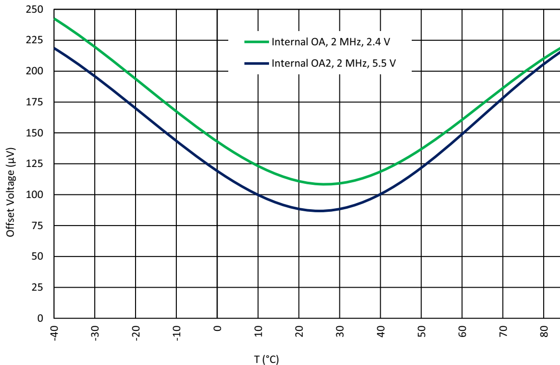
Figure 79: Internal Op Amp A_{at} Input CM Voltage = V_{DD}/2 , BW = 2 MHz
