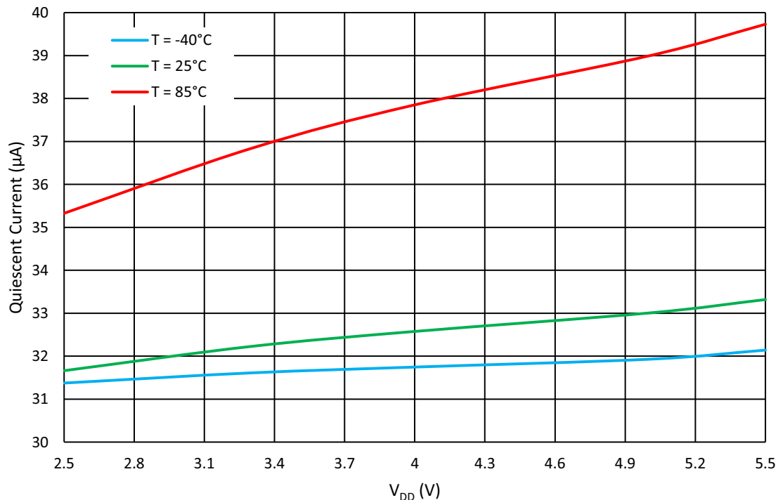
Figure 85: Quiescent Current vs. Power Supply Voltage for BW = 128\text{ kHz}
