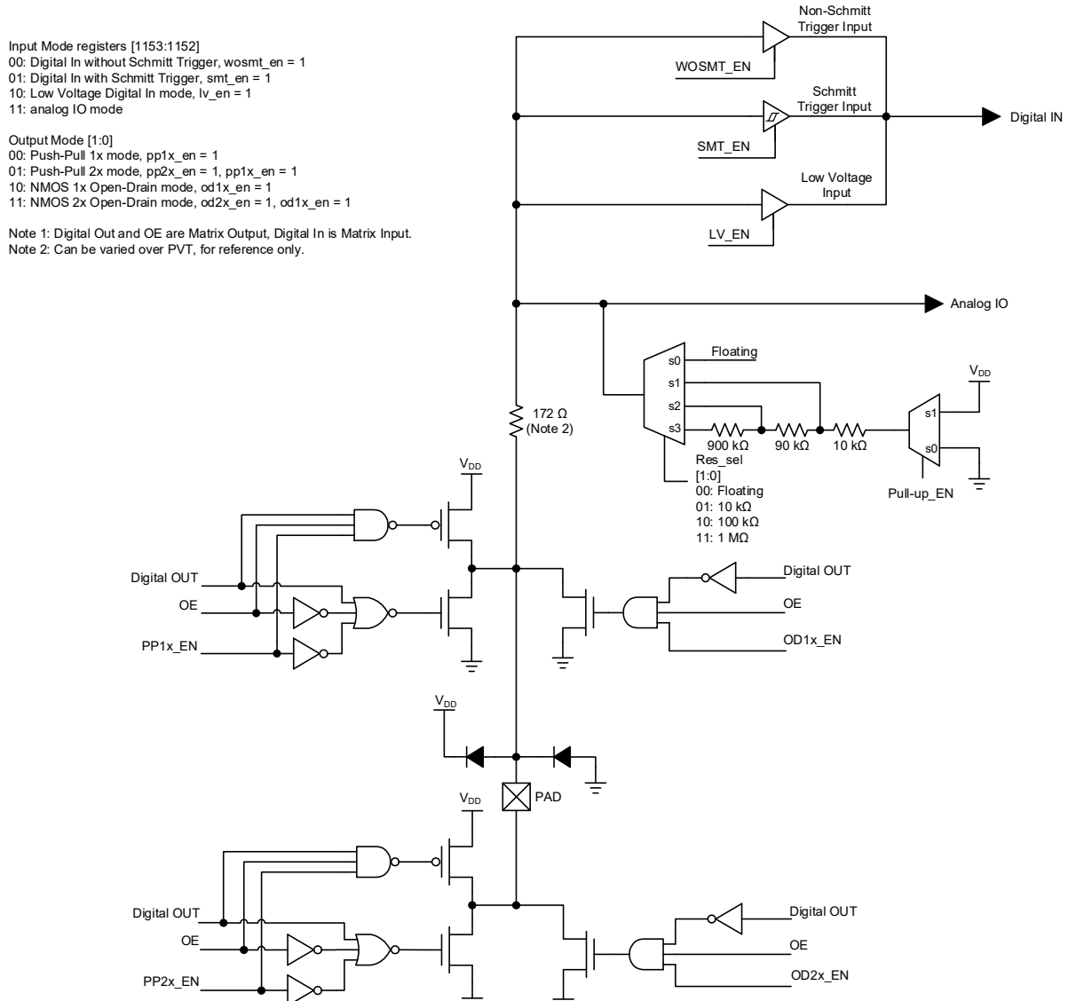
Figure 4: Matrix OE IO Structure Diagram
