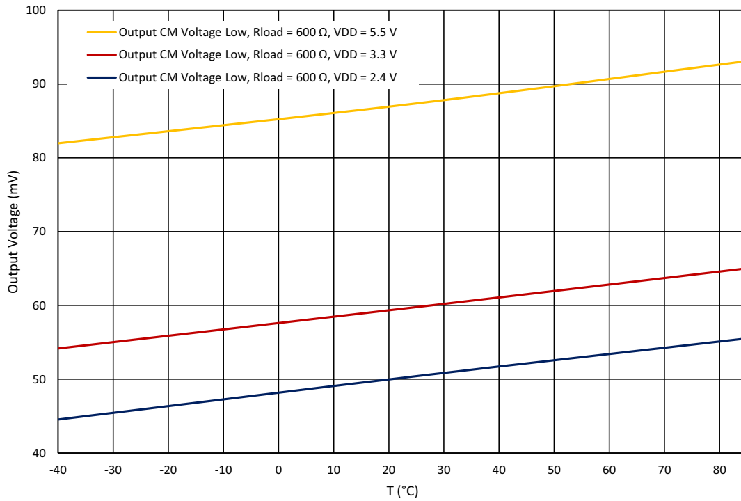
Figure 148: Output Voltage Low ( V_{\text{OUT}} - \text{GND} ) vs. Temperature at \text{BW} = 8\text{ MHz} , R_{\text{LOAD}} = 600\ \Omega
