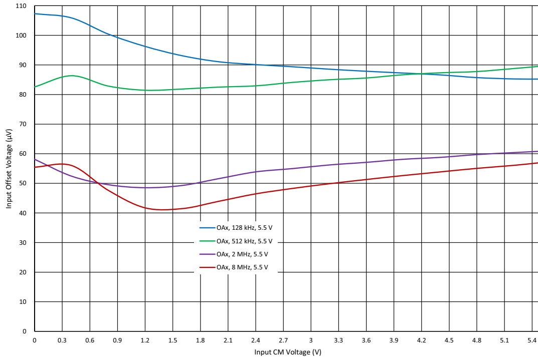
Figure 82: OpAmp0, 1 Input Offset Voltage vs. Input CM Voltage at T = 25^\circ\text{C} , V_{\text{DDA}} = 5.5\text{ V}
