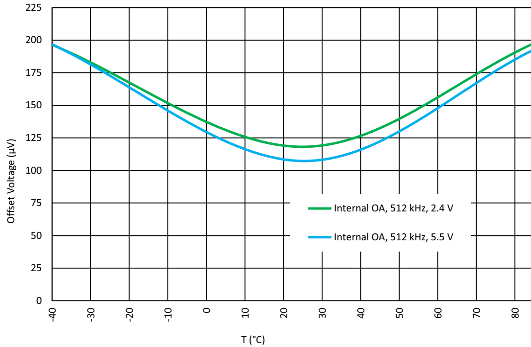
Figure 78: Internal Op Amp A_{at} Input CM Voltage = V_{DD}/2 , BW = 512 kHz
