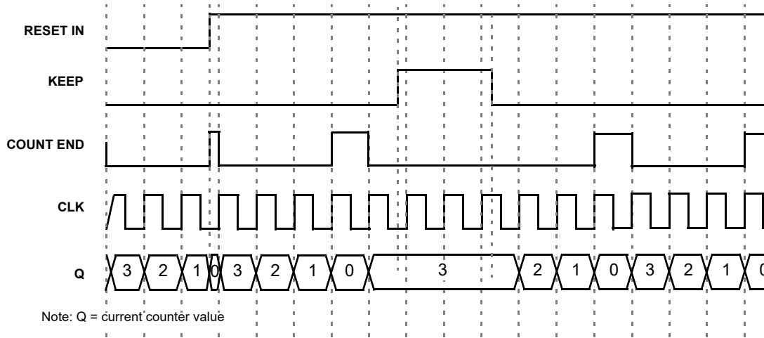
Figure 56: CNT/FSM Timing Diagram (Reset Rising Edge Mode, Oscillator is Forced On, UP = 0) for Counter Data = 3
