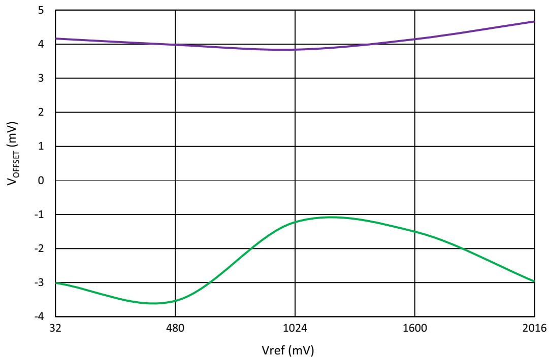
Figure 75: ACMPxL Input Offset Voltage vs. V_{ref} at T = -40\text{ }^{\circ}\text{C} to 105\text{ }^{\circ}\text{C}
