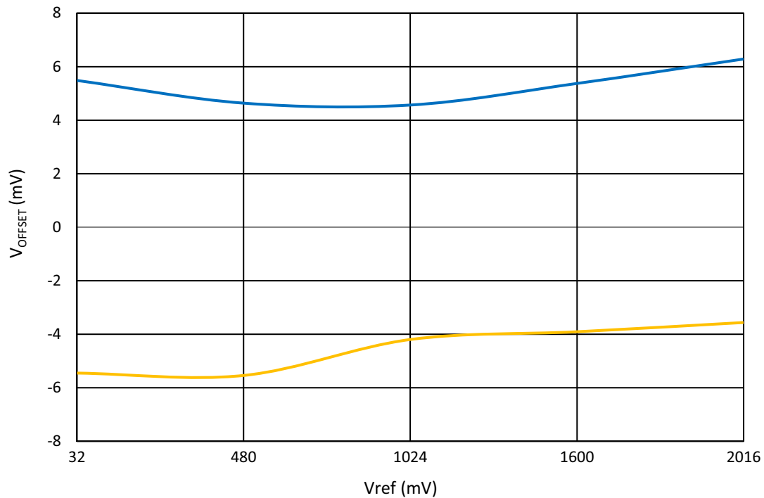
Figure 74: ACMPxH Input Offset Voltage vs. V_{ref} at T = -40\text{ }^{\circ}\text{C} to 105\text{ }^{\circ}\text{C}
