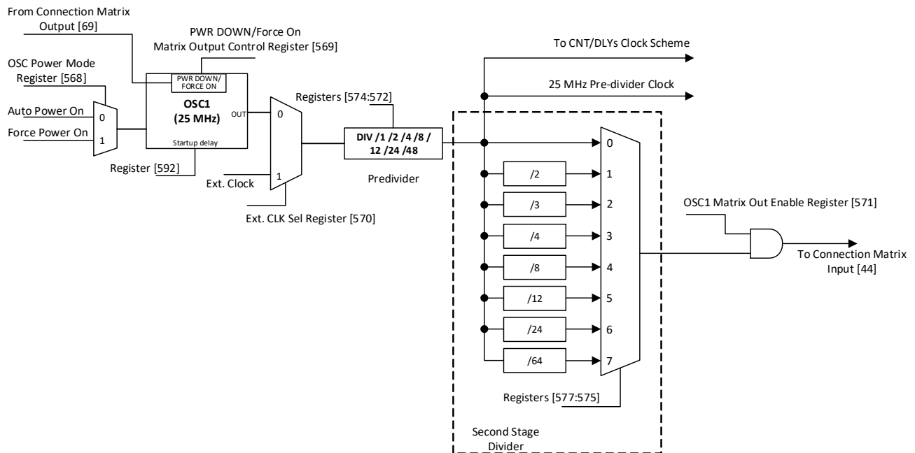
Figure 65: Oscillator1 Block Diagram
