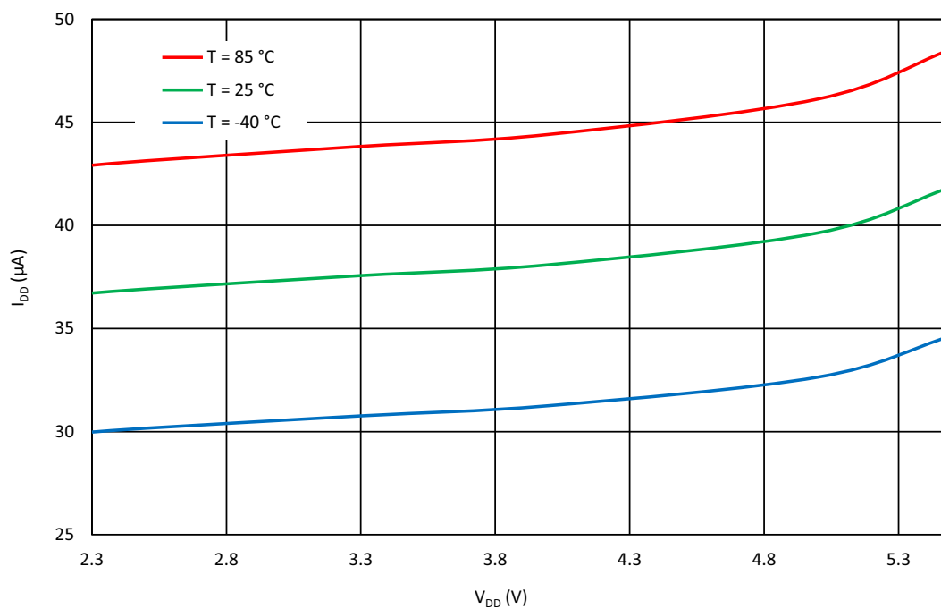
Figure 60: Current Consumption vs. V_{DD} for Sampling Mode, 4 Channels, V_{IN+} = 2048 \text{ mV} , V_{IN-} = 32 \text{ mV} , Clock = 10 kHz
