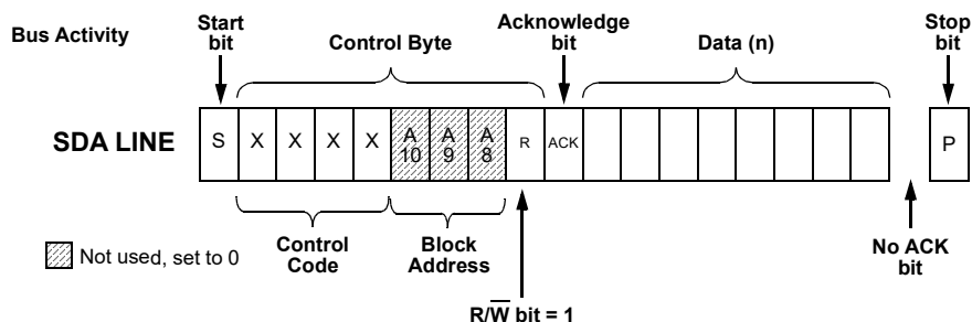
Figure 87: Current Address Read Command, R/\bar{W} = 1
