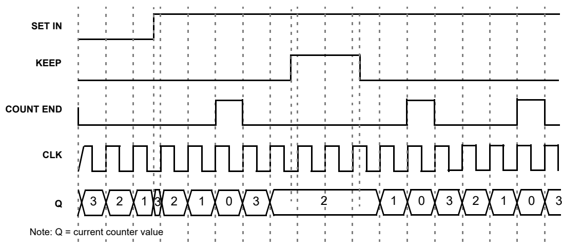
Figure 43. CNT/FSM Timing Diagram (set rising edge mode, oscillator is forced on, UP = 0) for counter data = 3
