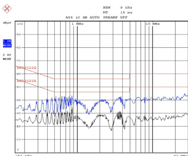
Figure 16. Neutral, 120V AC
