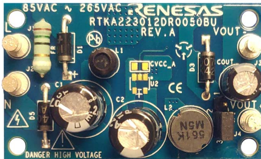
Figure 2. RTKA223012DR0050BU Evaluation Board (Top)
