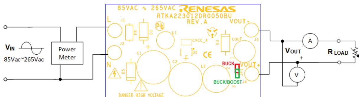
Figure 1. RTKA223012DR0050BU/RTKA223012DR0060BU Connection Diagram
