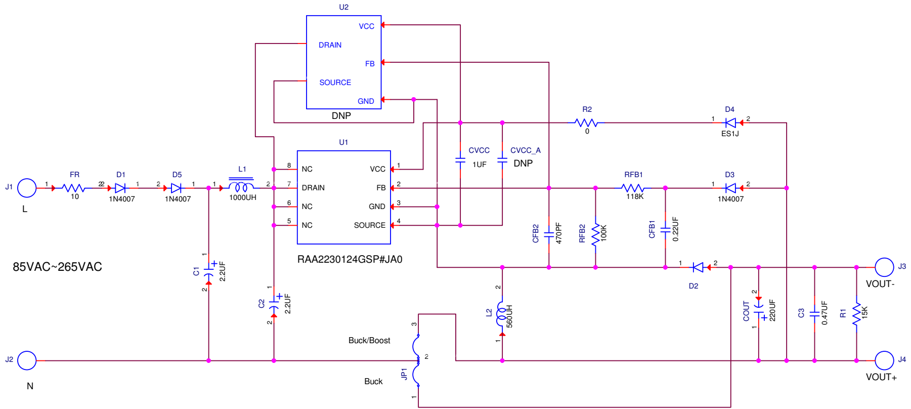
Figure 6. RTKA223012DR0050BU Schematic
