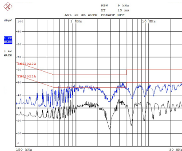
Figure 17. Neutral, 230V AC
