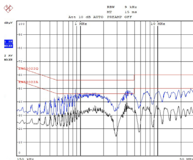
Figure 15. Line, 230V AC
