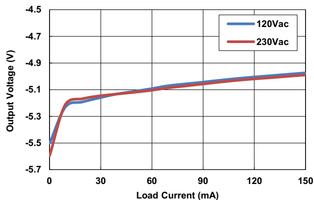
Figure 13. Load Regulation Buck/Boost
