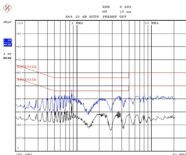
Figure 14. Line, 120V AC
