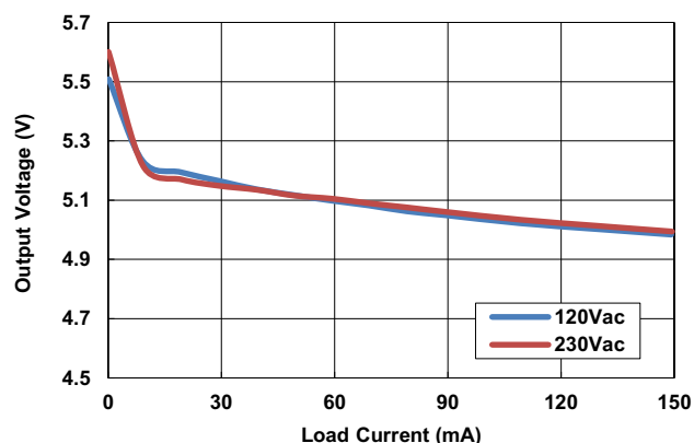
Figure 11. Load Regulation 5V Buck
