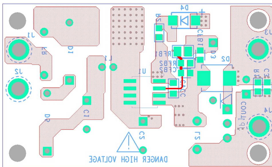
Figure 9. Bottom Layer
