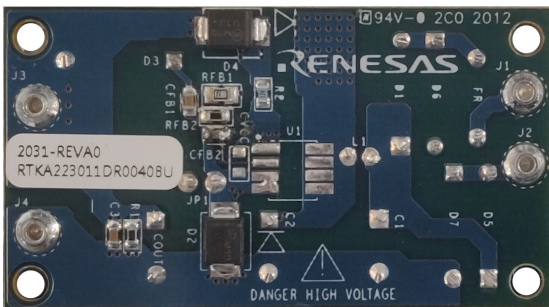
Figure 3. RTKA223011DR0040BU Evaluation Board (Bottom)
