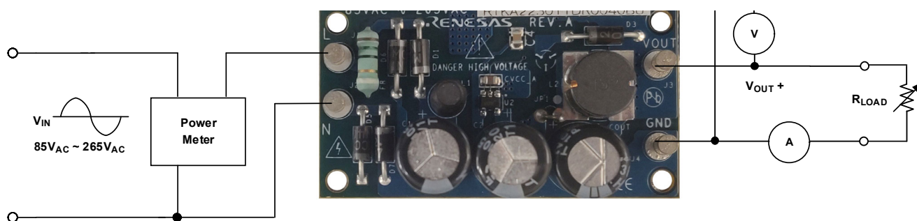
Figure 1. RTKA223011DR0040BU Connection Diagram
