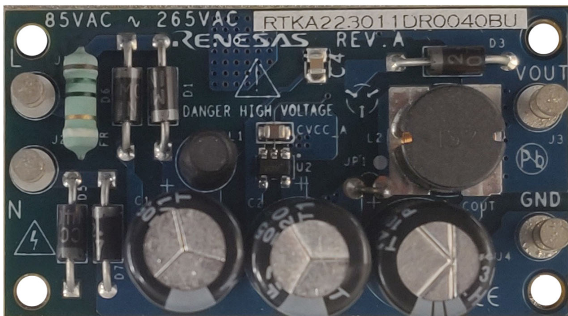
Figure 2. RTKA223011DR0040BU Evaluation Board (Top)
