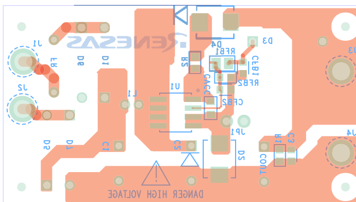
Figure 6. Bottom Layer
