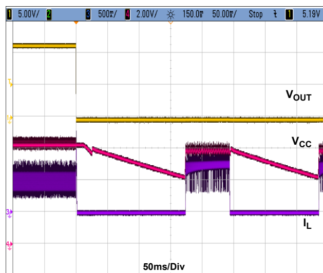
Figure 20. V_{IN} = 230V_{AC} , I_{OUT} = 0.5A to Short
