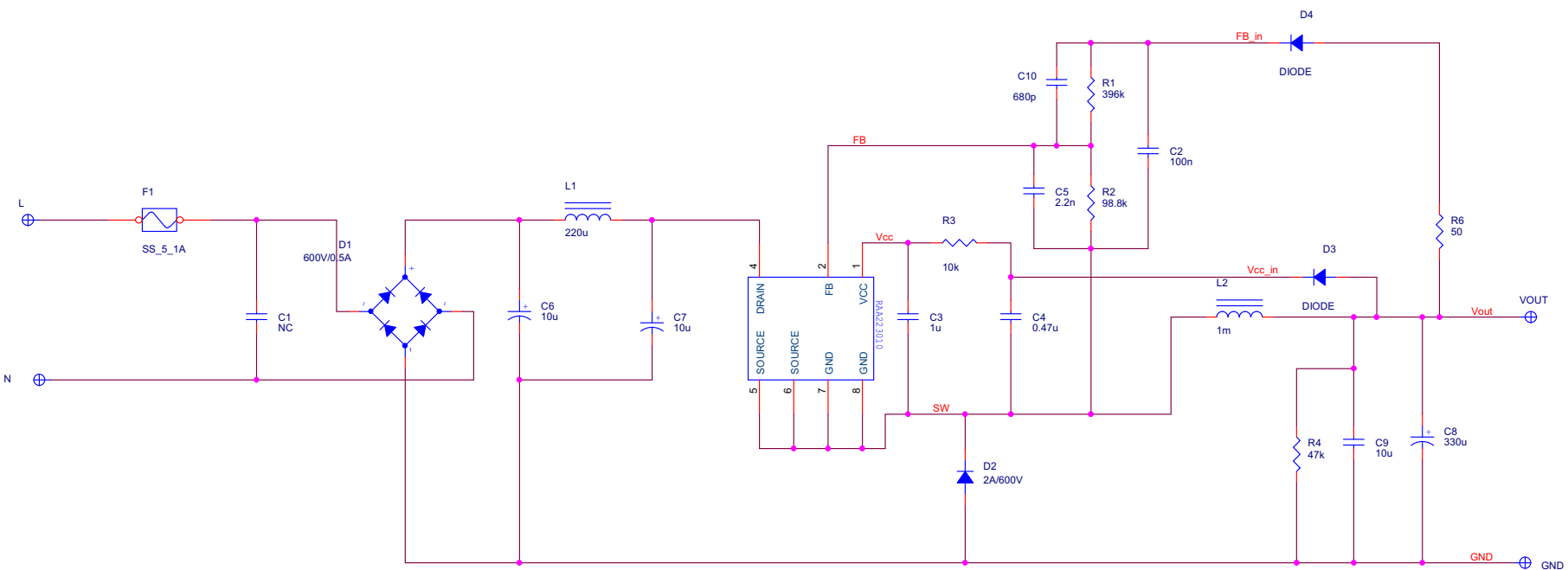
Figure 6. Schematic
