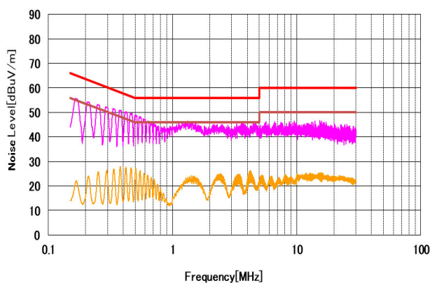
Figure 24. N Line, 230V AC
