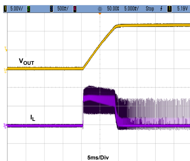
Figure 18. V_{IN} = 230V_{AC} , I_{OUT} = 0A
