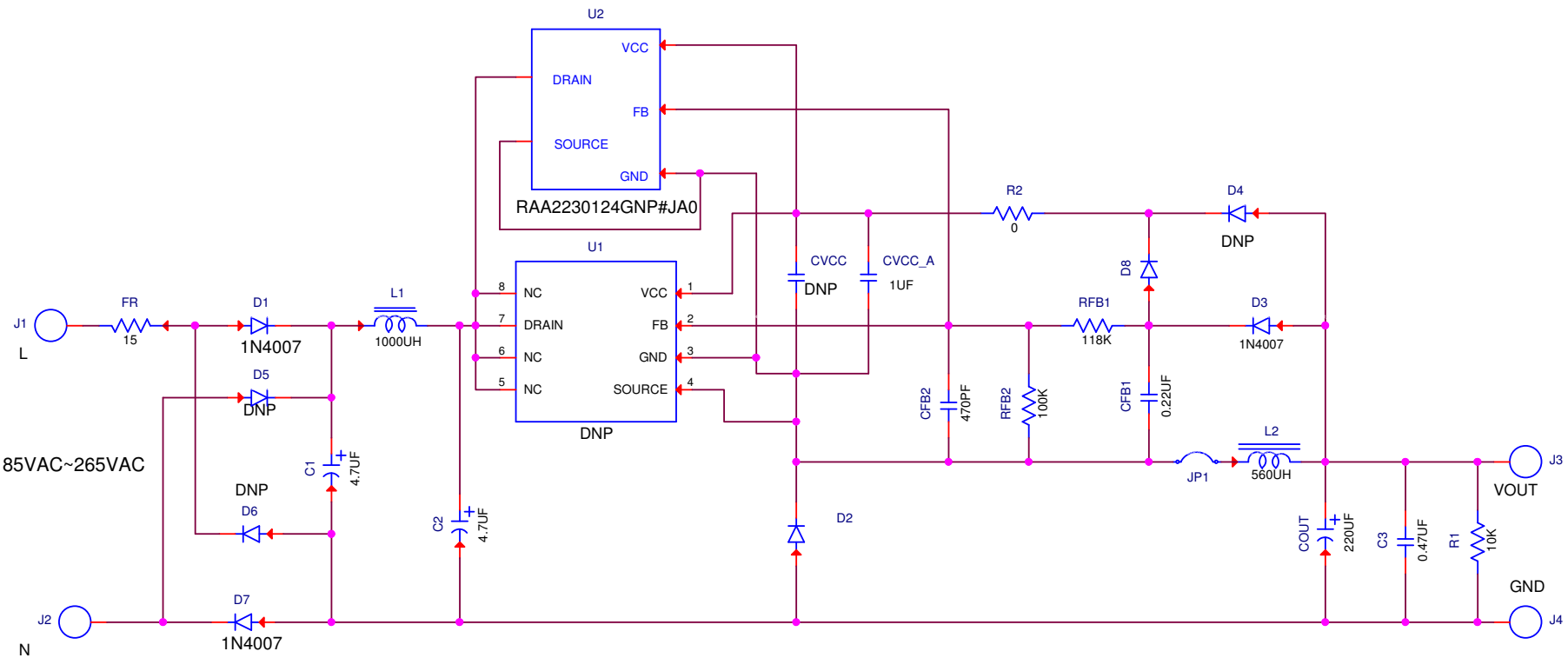
Figure 7. RTKA223012DR0020BU Schematic
