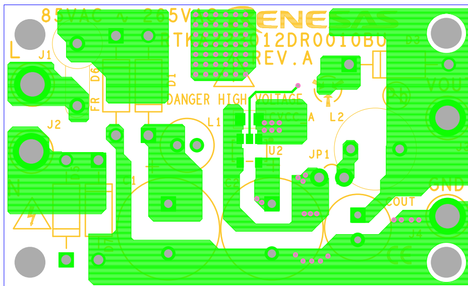
Figure 8. Top Layer
