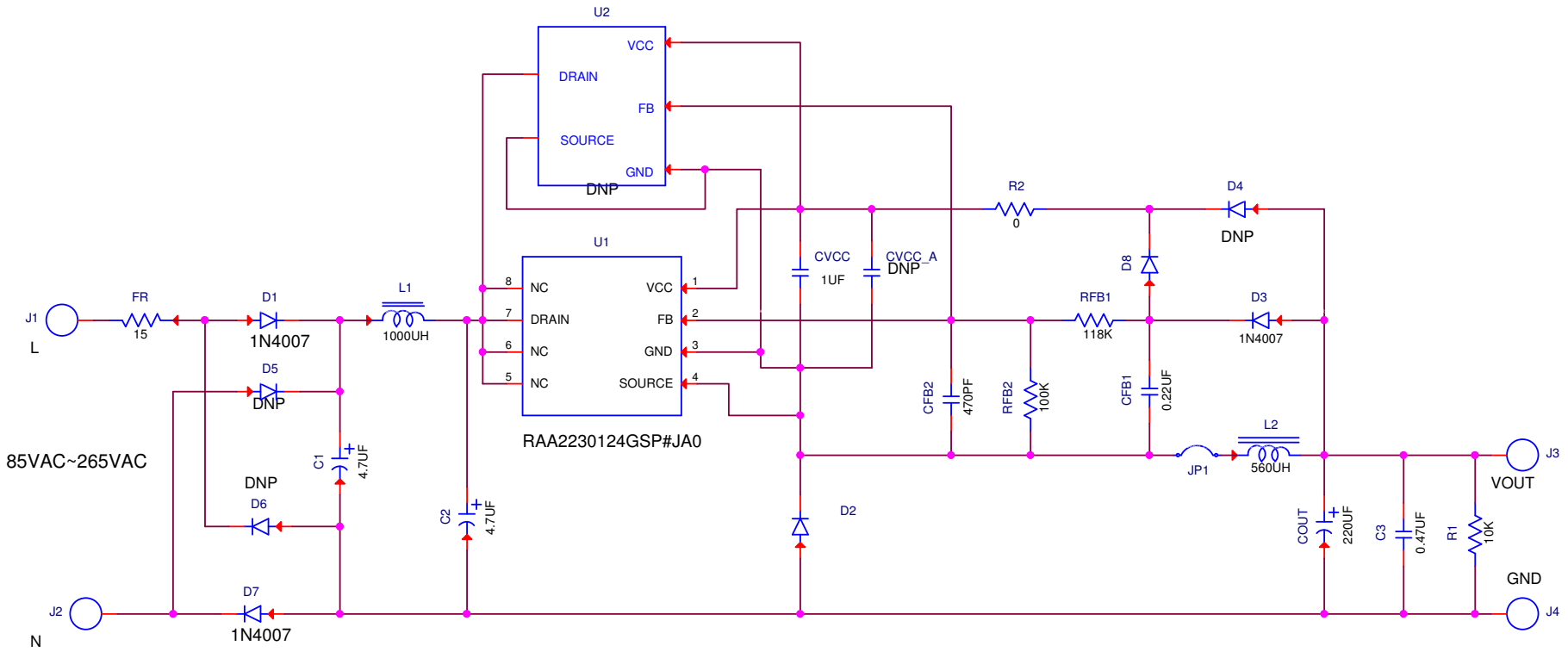
Figure 6. RTKA223012DR0010BU Schematic
