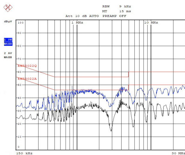
Figure 13. Line, 230V AC
