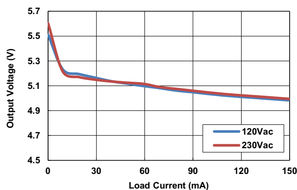
Figure 11. Load Regulation
