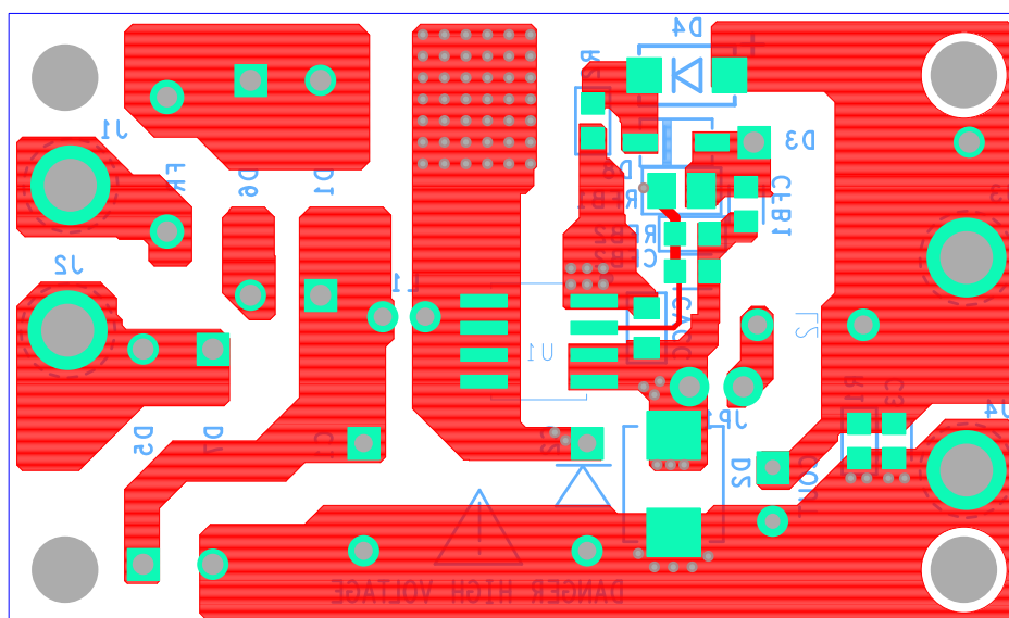
Figure 9. Bottom Layer
