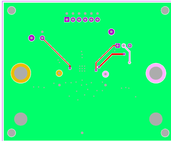
Figure 9. Bottom Layer
