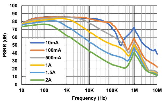
Figure 12. PSRR vs Frequency ( V_{IN} = 4\text{V} , V_{OUT} = 3.3\text{V} , C_{SET} = 1\mu\text{F} , C_{OUT} = 22\mu\text{F} )
