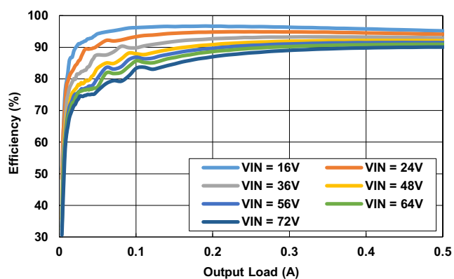
Figure 17. Efficiency
