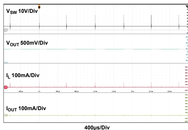
Figure 19. Buck Output Ripple at No Load
