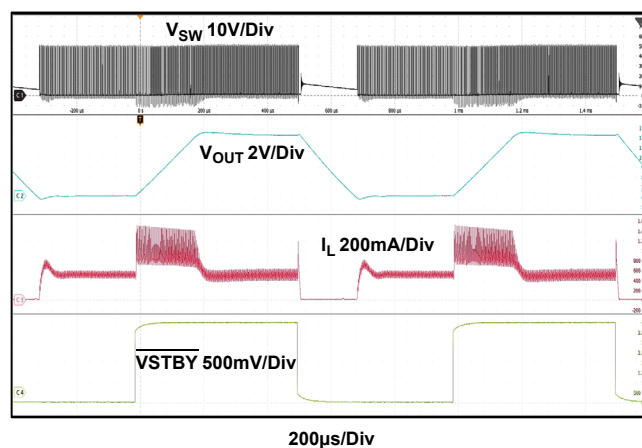
Figure 15. With External Standby Function at Full Load
