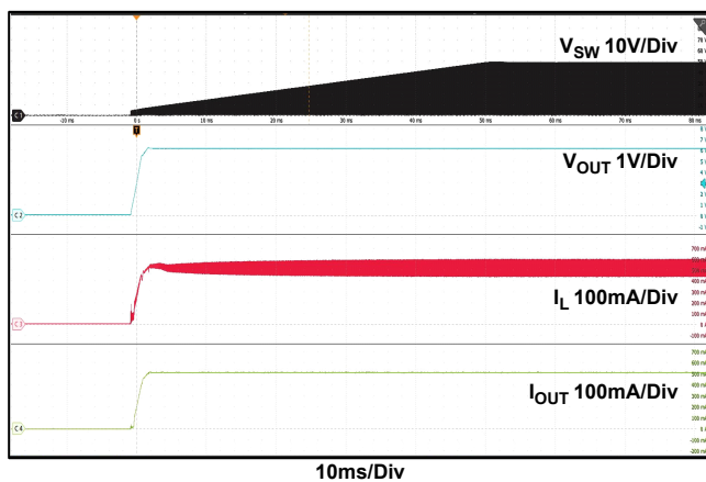
Figure 12. Power-On at Full Load
