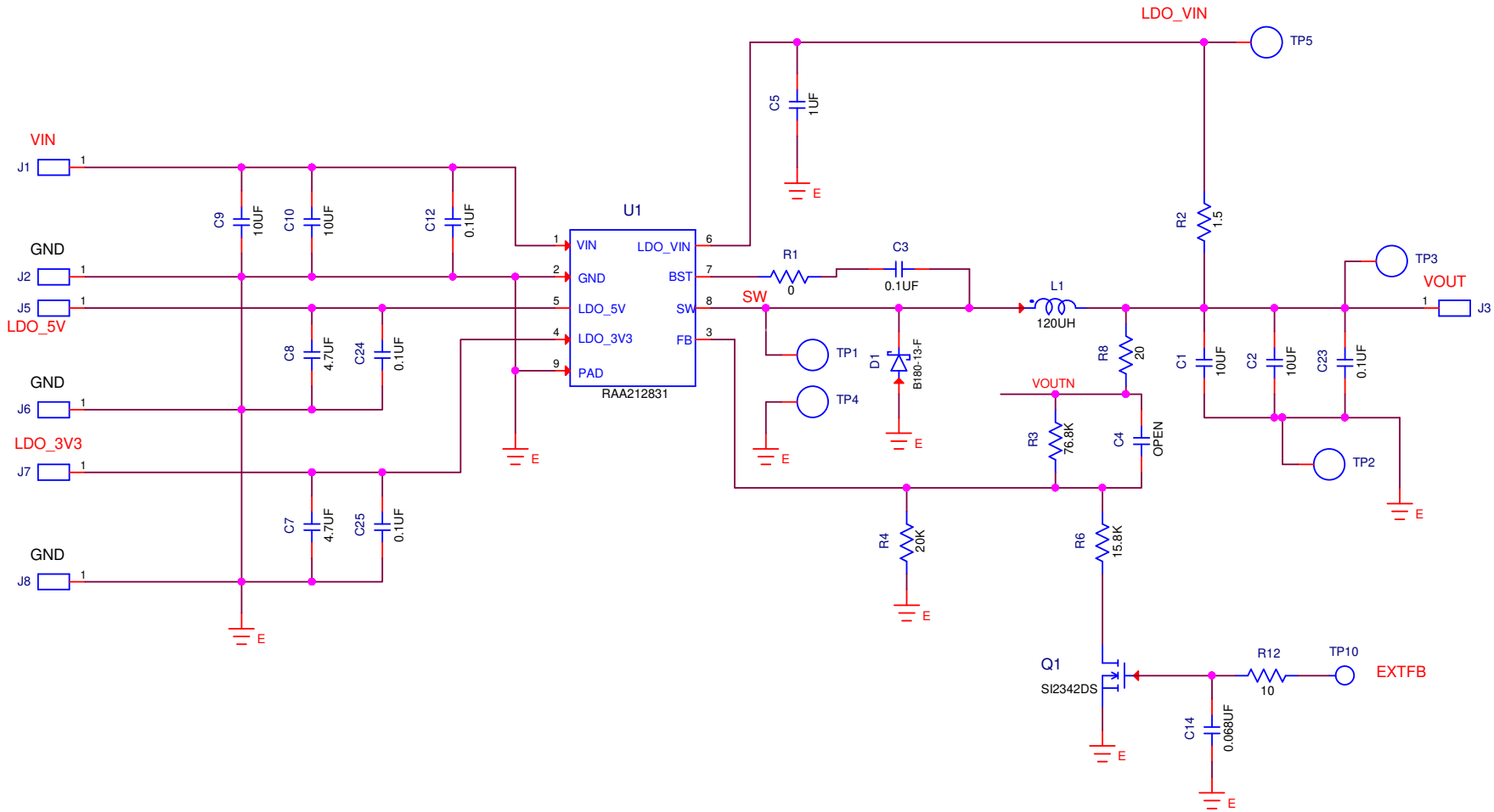
Figure 5. RTKA212831DR0000BU Board Circuit Schematic
