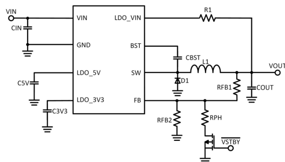
(b) with external standby function
