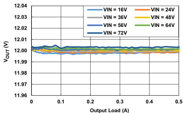
Figure 16. Load Regulation
