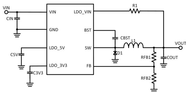
(a) Without External Standby Function
