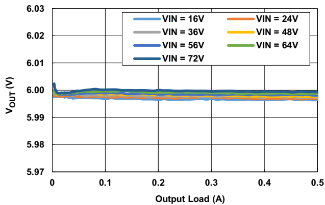
Figure 8. Load Regulation
