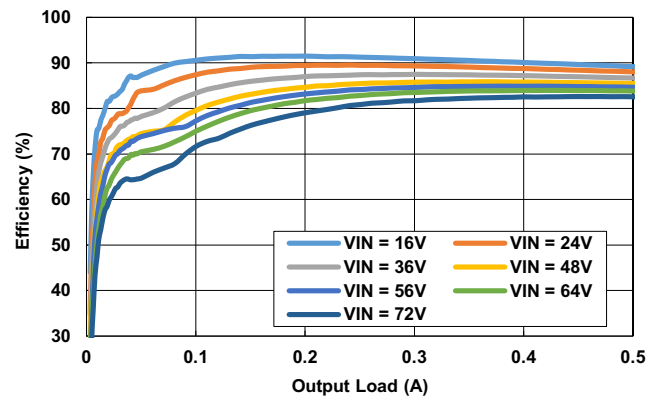
Figure 9. Efficiency
