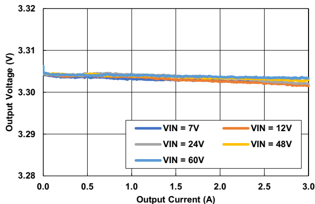
Figure 10. Load Regulation
