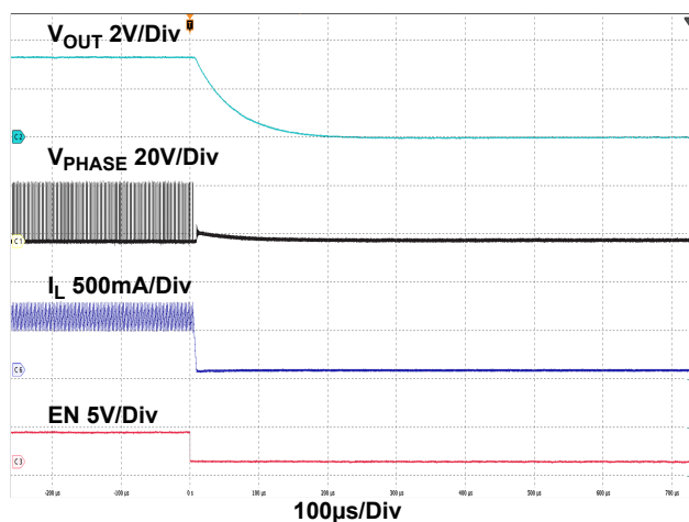
Figure 11. Enable Off at Full Load
