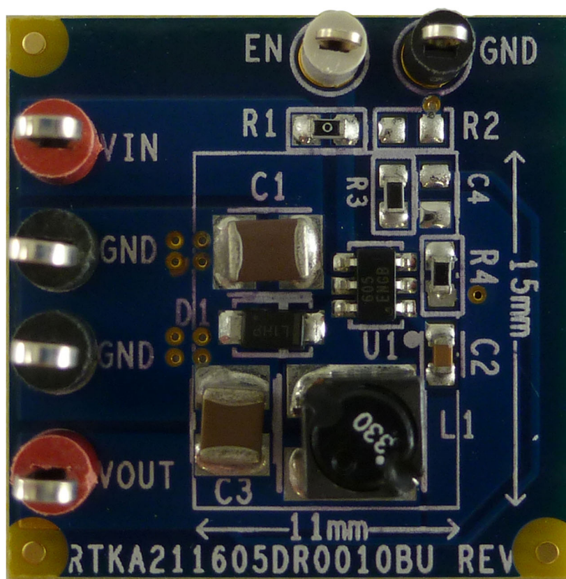
Figure 3. Top View
