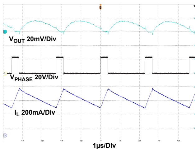
Figure 9. Output Ripple at Full Load
