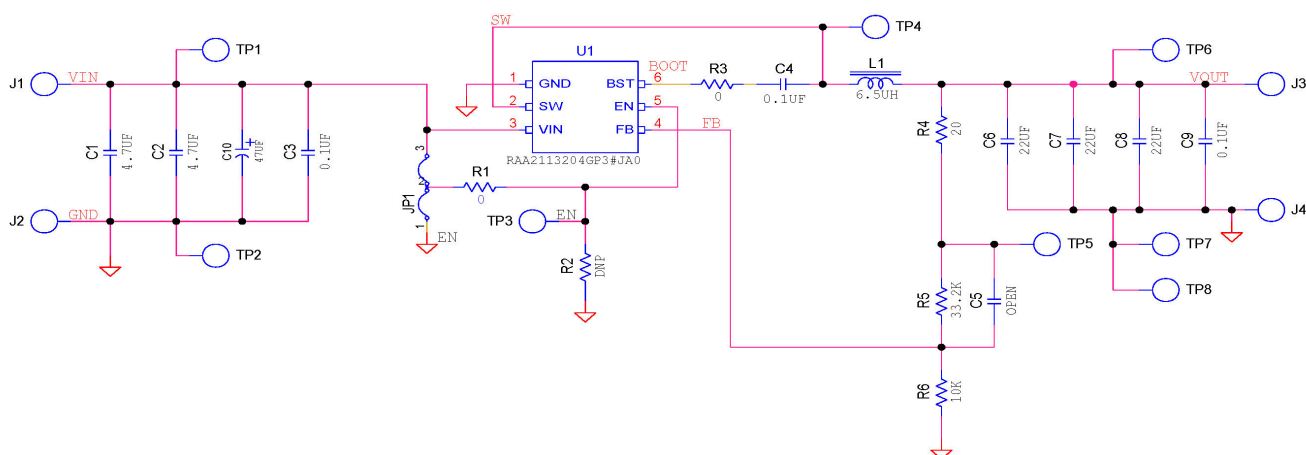
Figure 3. RTKA211320DE0030BU Schematic
