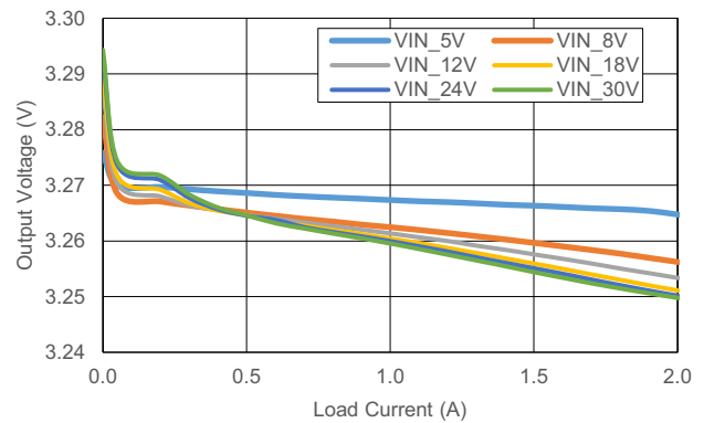
Figure 7. Load Regulation
