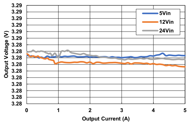
Figure 10. Load Regulation
