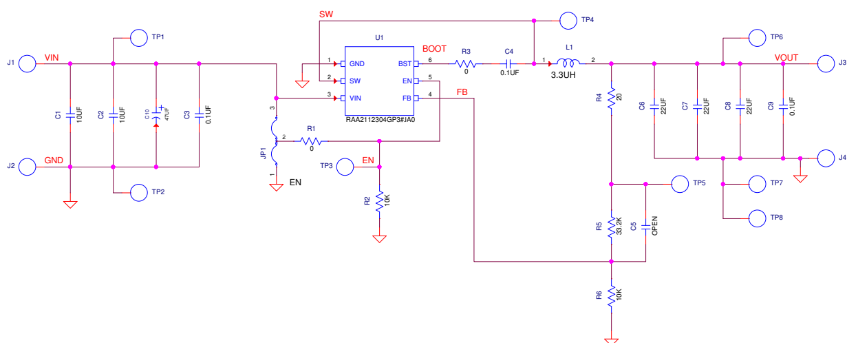
Figure 3. RTKA211230DE0020BU Schematic
