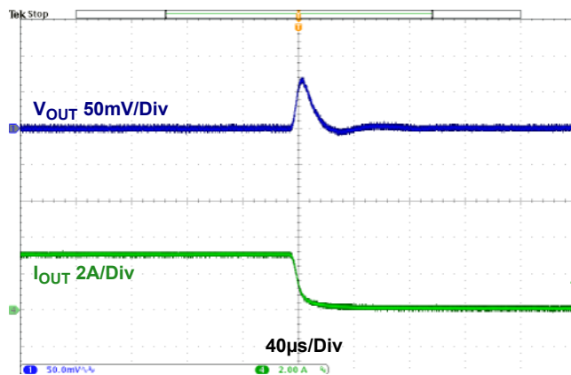
Figure 21. Transient Response, V_{IN} = 3.3V , V_{OUT} = 1.8V , f_{SW} = 2MHz , 3A to 0A, C_{OUT} = 2x22\mu F Ceramic, FPWM
