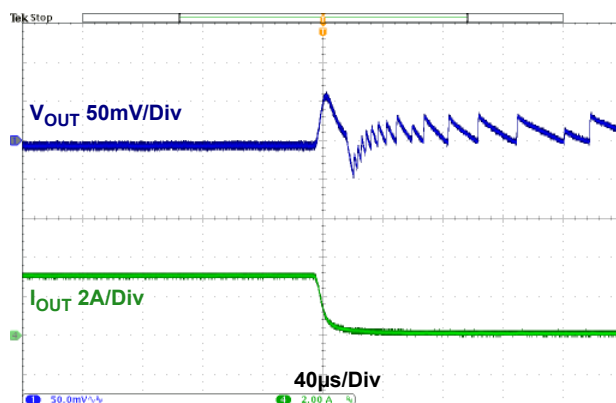
Figure 27. Transient Response, V_{IN} = 5V , V_{OUT} = 1.8V , f_{SW} = 2MHz , 3A to 0A , C_{OUT} = 2x22\mu F Ceramic, PFM
