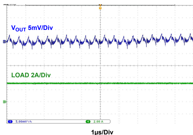
Figure 18. Output Ripple, V_{IN} = 3.3V , V_{OUT} = 1.8V , f_{SW} = 2MHz , Full Load, C_{OUT} = 2 \times 22\mu F Ceramic
