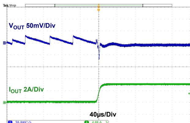
Figure 26. Transient Response, V_{IN} = 5V , V_{OUT} = 1.8V , f_{SW} = 2MHz , 0A to 3A , C_{OUT} = 2x22\mu F Ceramic, PFM
