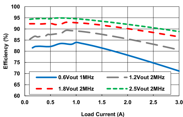
Figure 16. Efficiency vs Load Current, PFM, V_{IN} = 3.3V
