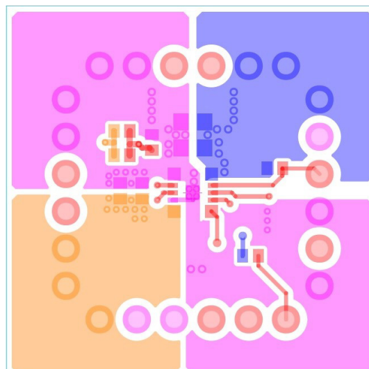
Figure 9. Top Layer
