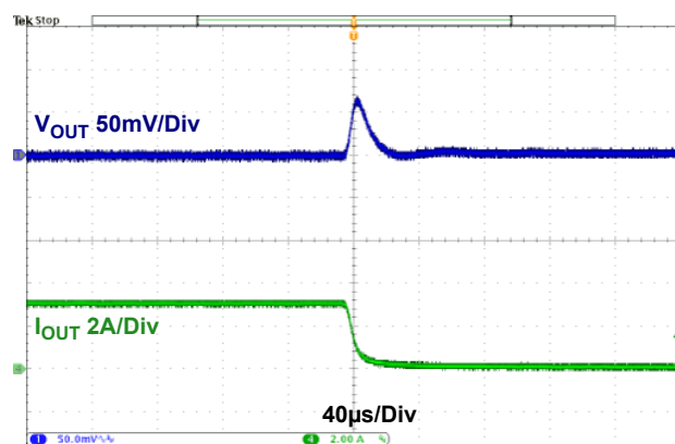
Figure 23. Transient Response, V_{IN} = 5V , V_{OUT} = 1.8V , f_{SW} = 2MHz , 3A to 0A, C_{OUT} = 2x22\mu F Ceramic, FPWM
