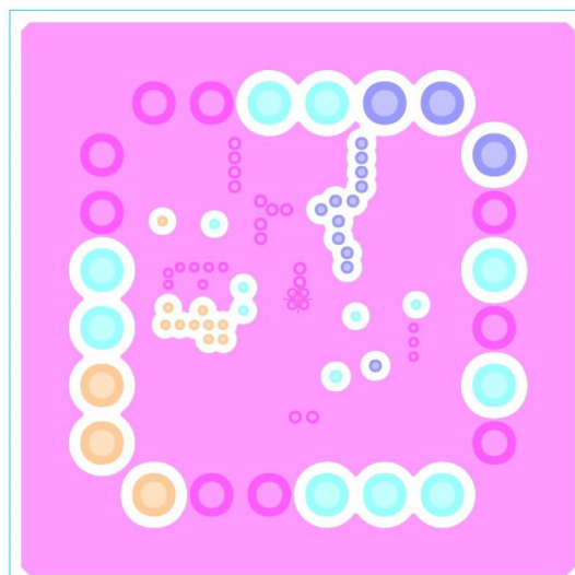
Figure 11. Layer 3
