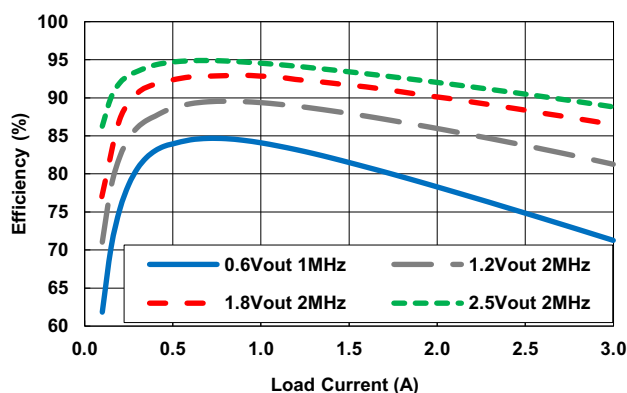
Figure 14. Efficiency vs Load Current, PWM, V_{IN} = 3.3V
