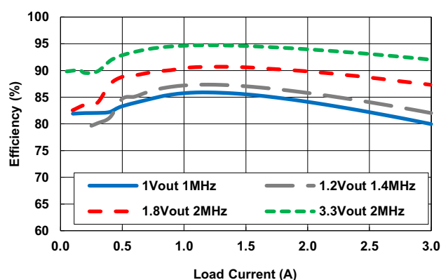
Figure 17. Efficiency vs Load Current, PFM, V_{IN} = 5V
