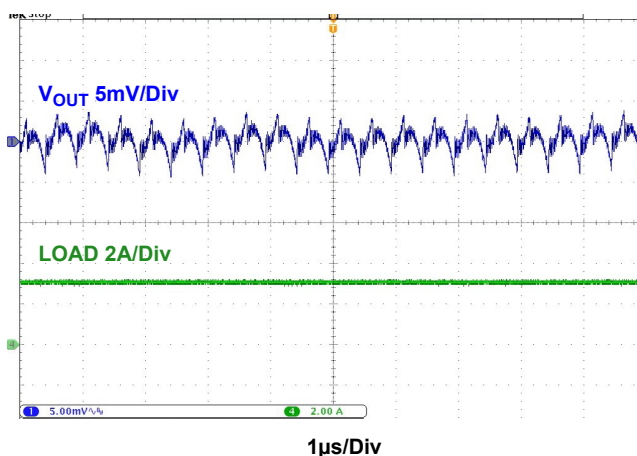
Figure 19. Output Ripple, V_{IN} = 5V , V_{OUT} = 1.8V , f_{SW} = 2MHz , Full Load, C_{OUT} = 2 \times 22\mu F Ceramic
