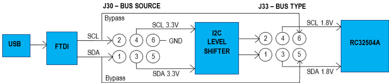
Figure 4. Communication Path Block Diagram
