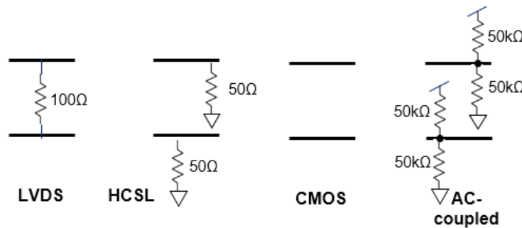
Figure 6. Input Buffer Behavior by Protocol
