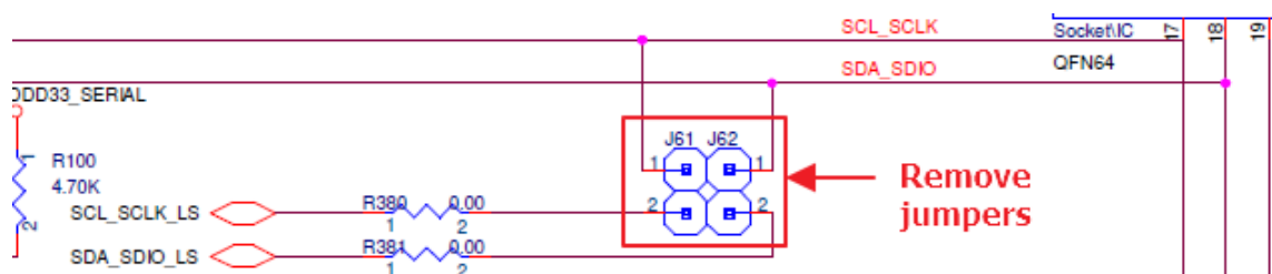
Figure 21. FTDI to I 2 C Communication Jumpers
