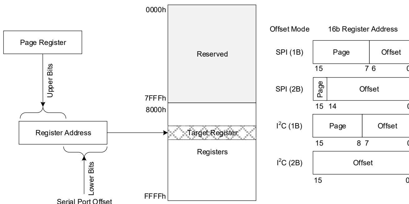
Figure 7. Register Addressing Modes via Serial Port
