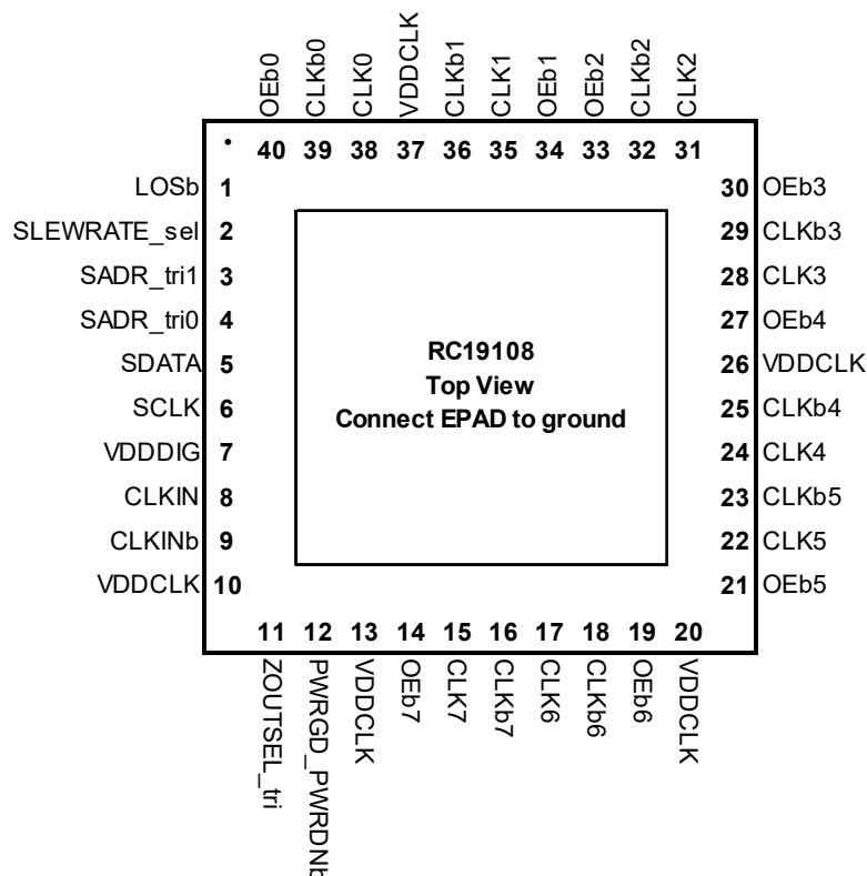
Figure 2. RC19108 40-VFQFP – Top View
