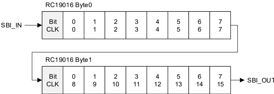
Figure 30. RC19016 Side-Band Shift Order
