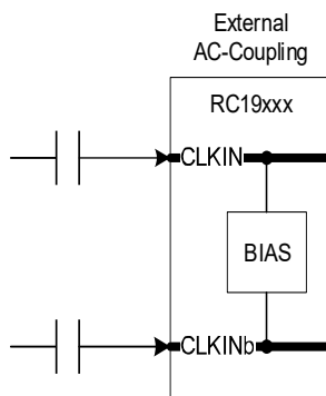
Figure 18. External AC-Coupling
