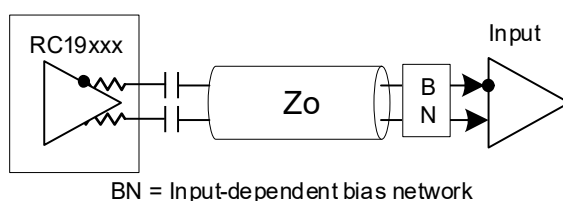
Figure 22. AC-Coupled
