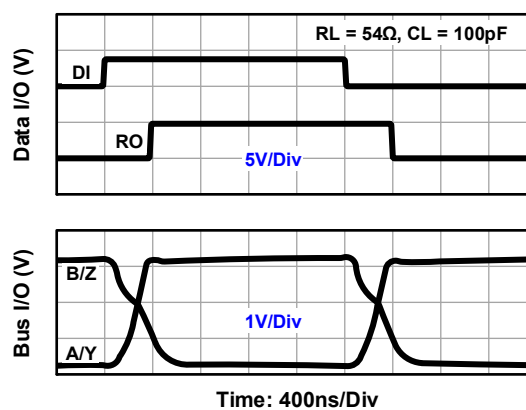
Figure 19. Waveforms (RAA788153, RAA788155)
