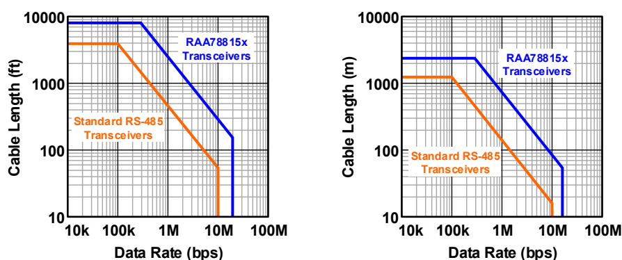
Figure 34. Data Rate vs Cable Length Guidelines in Feet and Meters
