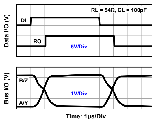
Figure 17. Waveforms (RAA788150, RAA788152)
