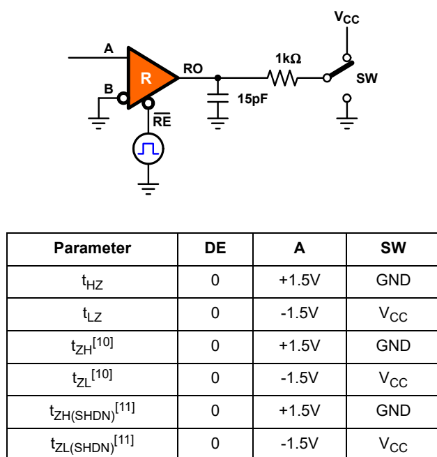
Figure 9. Measurement of Receiver Enable and Disable Times
