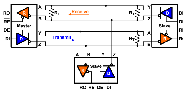
Figure 32. Full-Duplex Bus
