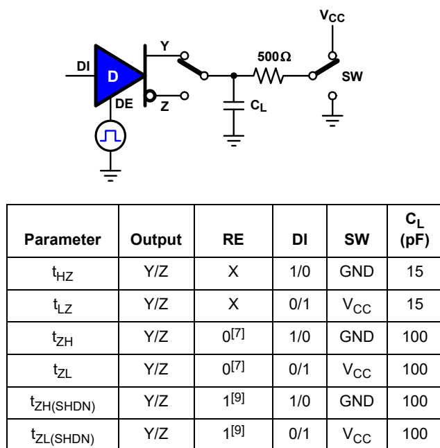
Figure 6. Measurement of Driver Enable and Disable Times
