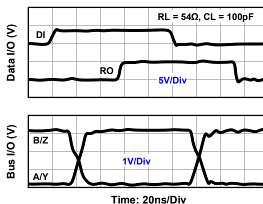
Figure 21. Waveforms (RAA788156, RAA788158)
