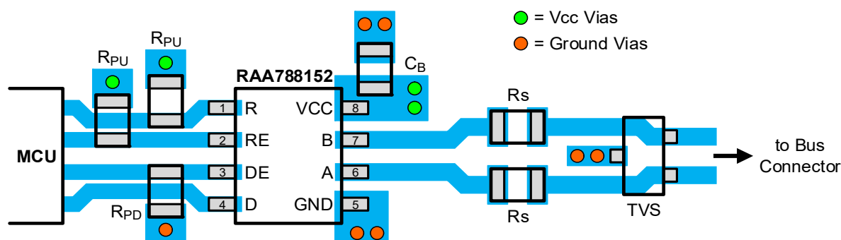
Figure 40. RAA788152 Layout Example
