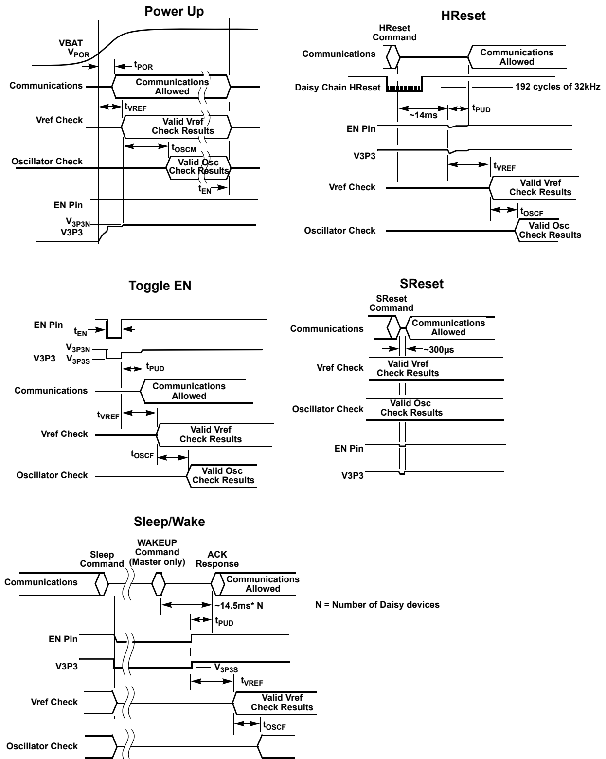
Figure 75. Power Sequencing
