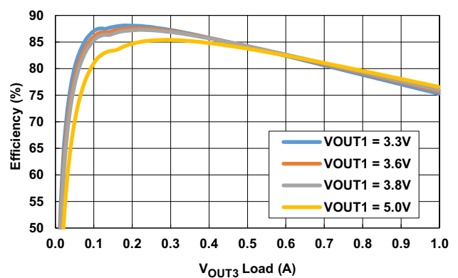
Figure 6. V_{OUT1} to V_{OUT3} = 1.2V , Efficiency vs Load
