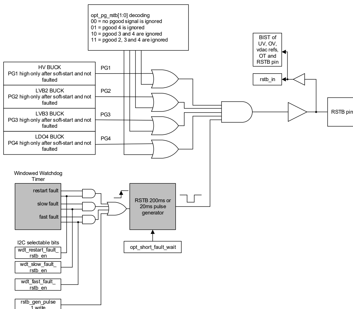
Figure 26. RSTB Block Diagram
