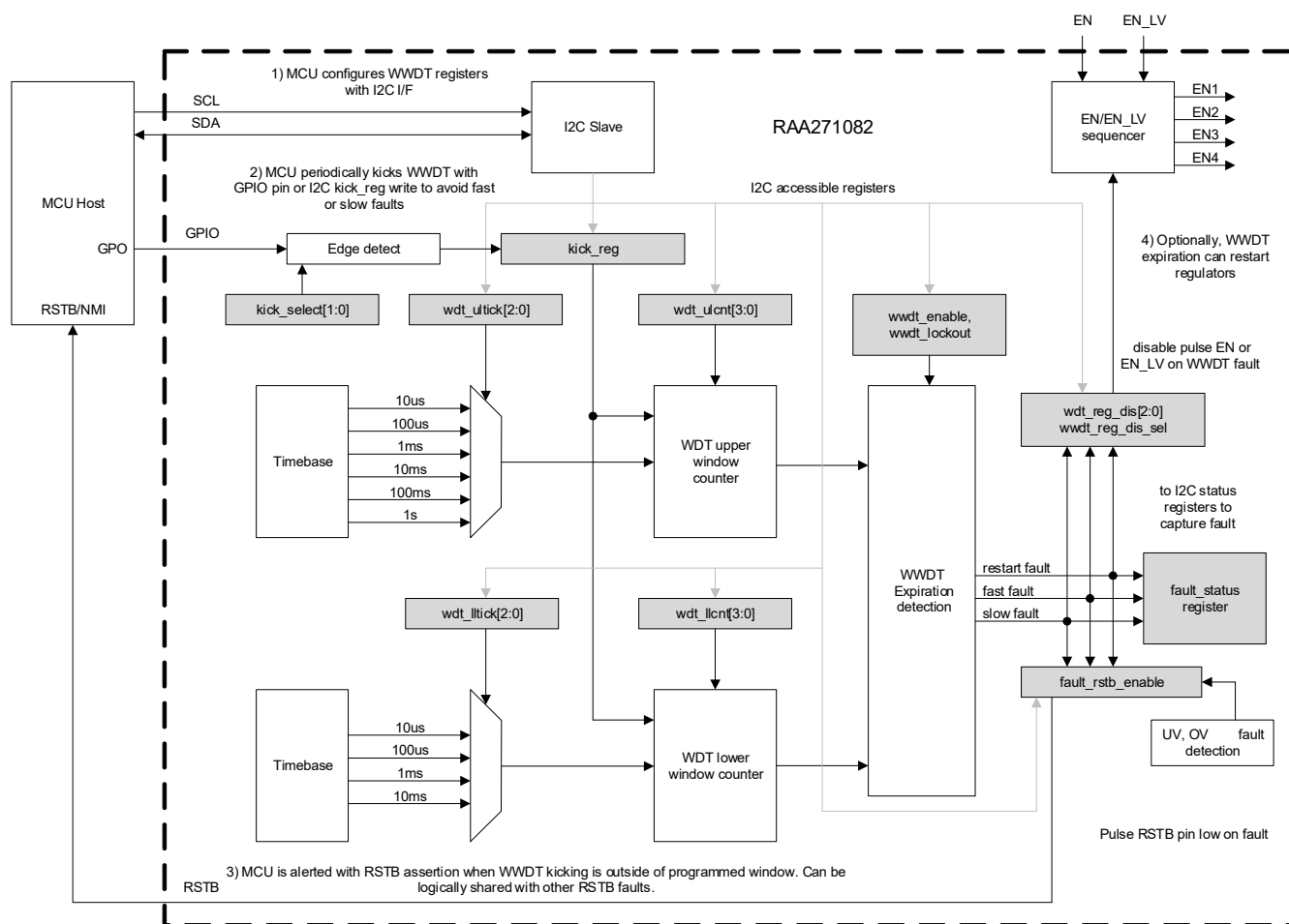
Figure 28. WWDT Operation using GPIO as WWDT Input
