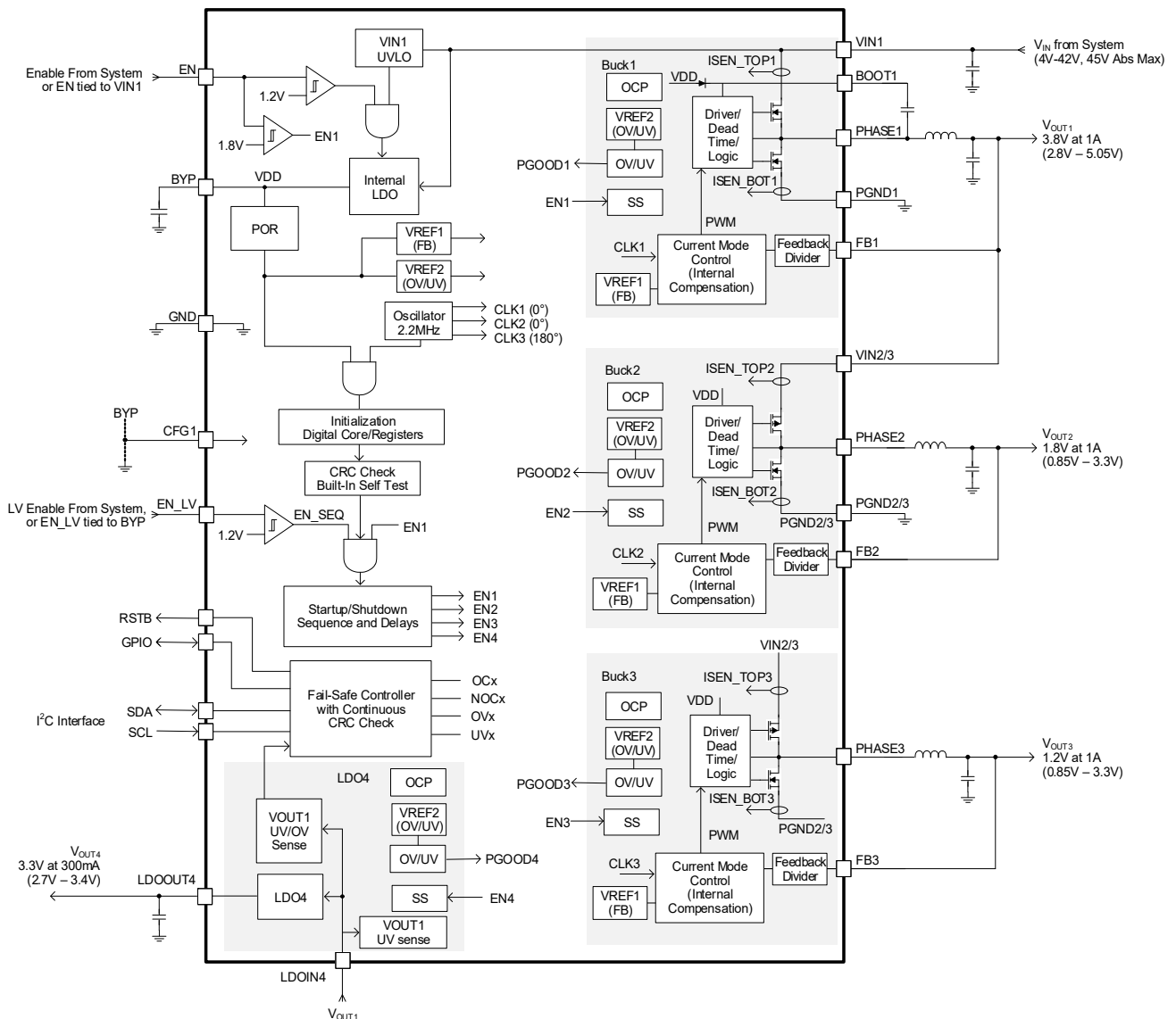
Figure 2. Block Diagram
