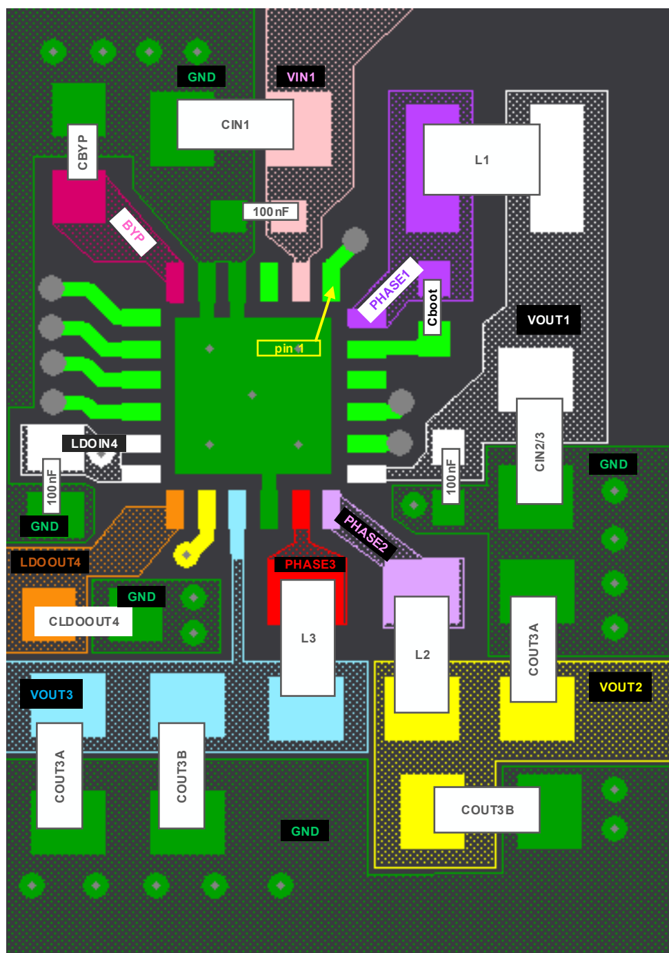
Figure 30. PCB Layout
