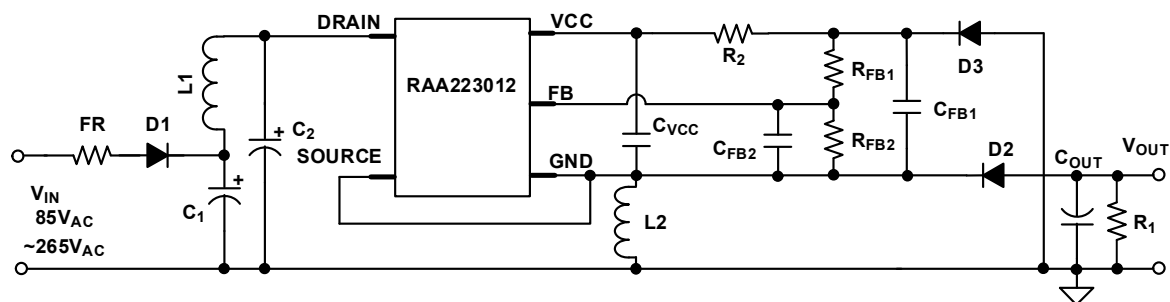
Figure 31. RAA223012 Buck/Boost
