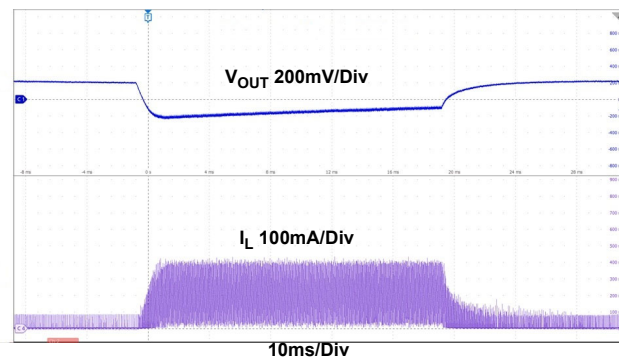
Figure 18. Load Transient (10mA to 250mA)
