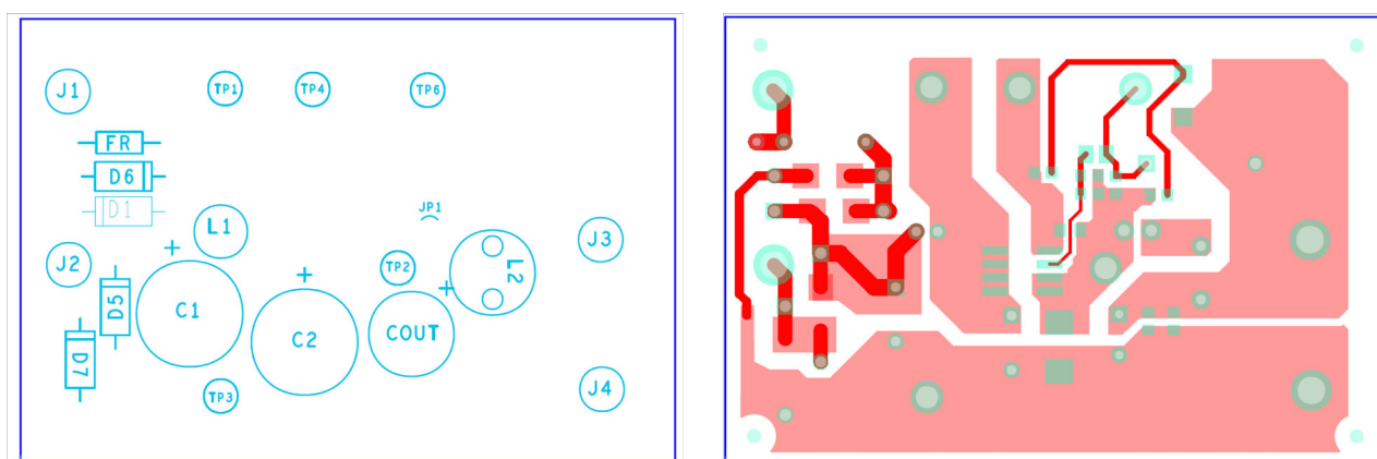
Figure 34. Example PCB Layout
