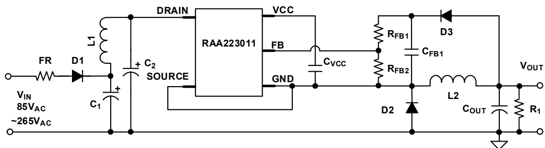
Figure 30. RAA223011 Buck with Low BOM Cost
