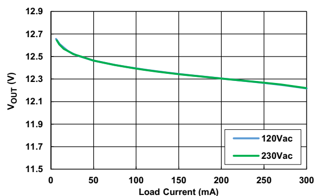
Figure 20. Load Regulation
