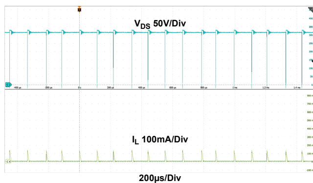
Figure 14. Light-Load Operation
