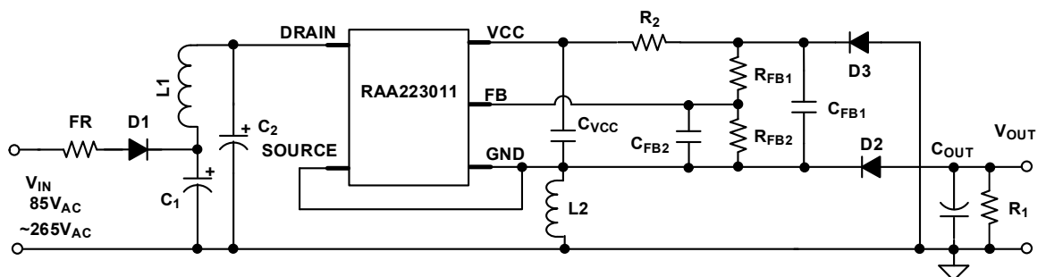
Figure 31. RAA223011 Buck/Boost
