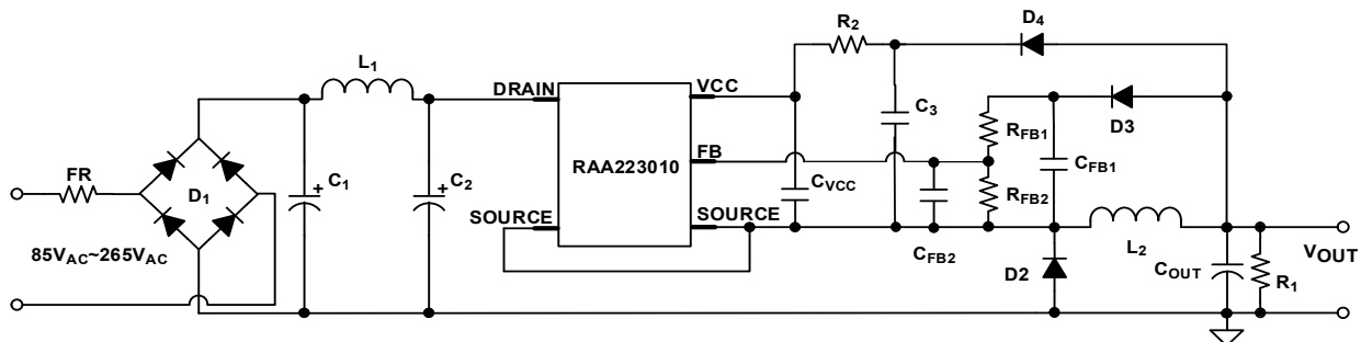
Figure 24. RAA223010 Low Standby Power Buck Regulator
