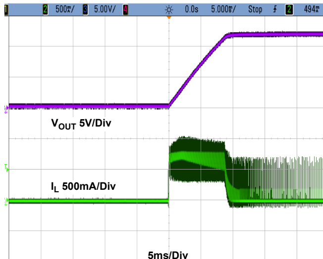
Figure 12. Startup ( V_{\text{IN}} = 230\text{V}_{\text{AC}} , No Load)
