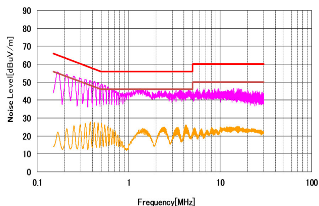
Figure 35. CE Line, 220V AC
