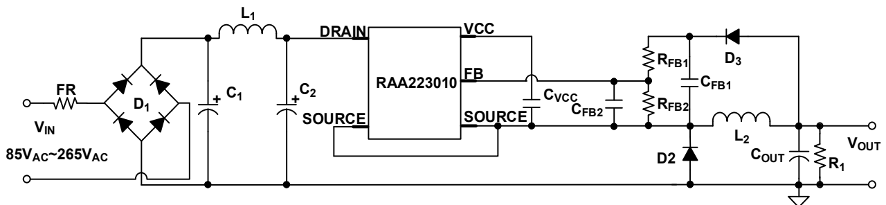
Figure 30. RAA223010 Buck with 3.3V Output
