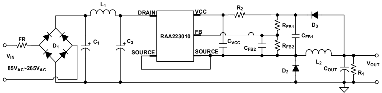
Figure 28. RAA223010 Buck with VCC Backfeed from C_{FB1}
