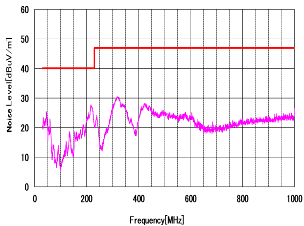
Figure 38. RE, Horizontal, 220V AC
