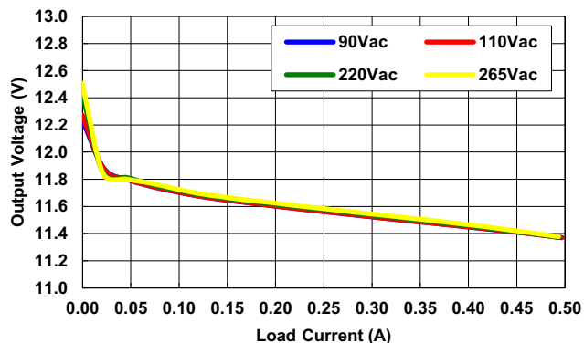
Figure 20. Load Regulation
