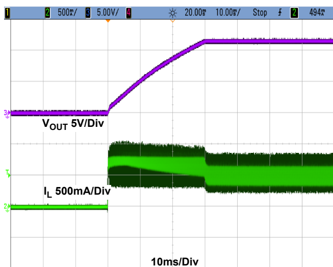
Figure 11. Startup ( V_{\text{IN}} = 230\text{V}_{\text{AC}} )
