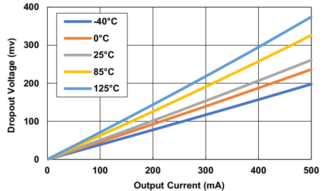
Figure 22. Dropout Voltage vs Output Current for Various Junction Temperatures ( V_{IN} = 20V )
