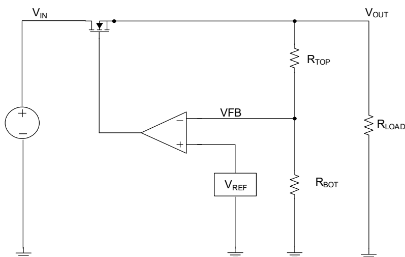
Figure 42. Simple NMOS LDO Regulator Block Diagram
