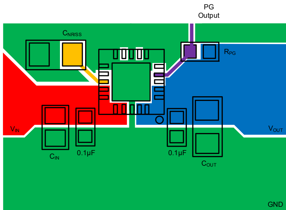
Figure 55. Layout Example
