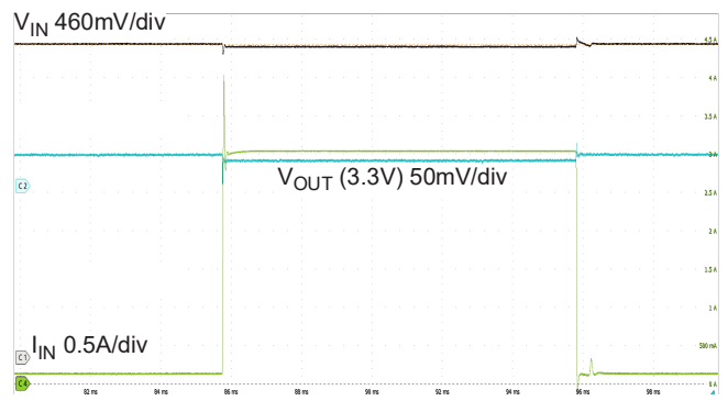
Figure 22. Load Transient Response ( V_{IN} = 3.7\text{V} , V_{OUT} = 3.3\text{V} , \Delta I_{OUT} = 0.1\text{A} to 3\text{A} at 1\text{A}/\mu\text{s} )
