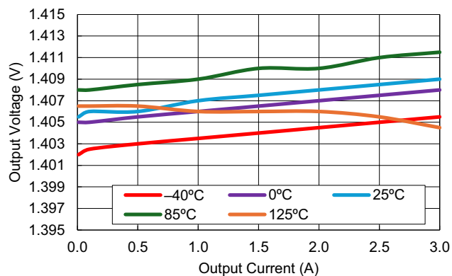
Figure 28. Load Regulation vs Output Current ( V_{OUT} = 1.4\text{V} )
