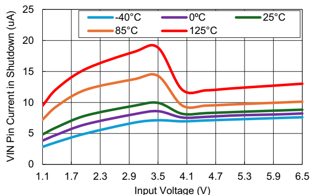
Figure 40. Shutdown Current vs Input Voltage for Various Temperatures
