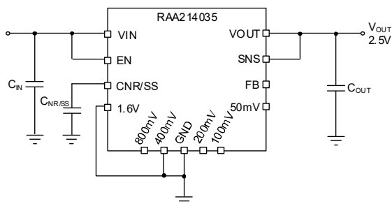
Figure 50. Internal FB Resistor Configuration for 2.5V ( V_{OUT} = 0.5V_{REF} + 1.6V + 400mV )
