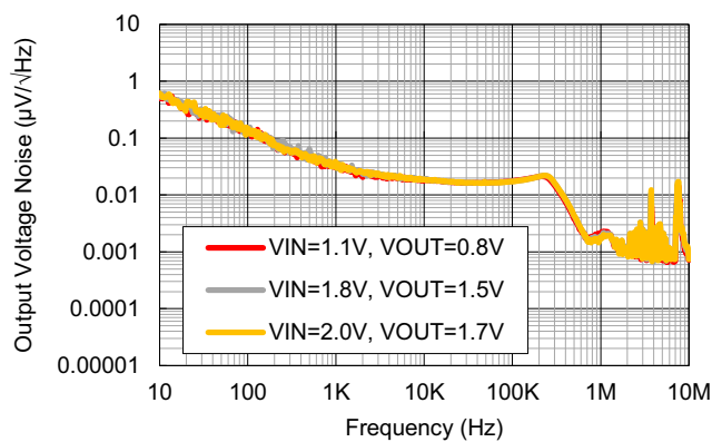
Figure 11. Output Voltage Noise for Various V_{OUT} ( V_{IN} = V_{OUT} + 0.3\text{V} , V_{BIAS} = 5\text{V} , I_{OUT} = 3\text{A} )
