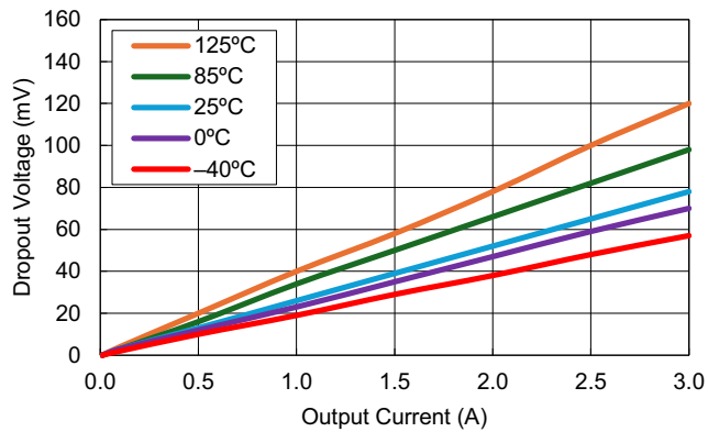
Figure 23. Dropout Voltage vs Output Current ( V_{OUT} = 1.1\text{V} )
