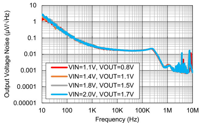
Figure 9. Output Voltage Noise for Various V_{OUT} ( V_{IN} = V_{OUT} + 0.3\text{V} , V_{BIAS} = 5\text{V} , I_{OUT} = 3\text{A} , C_{NR/SS} = 0.1\mu\text{F} )
