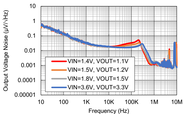
Figure 10. Output Voltage Noise for Various V_{OUT} ( V_{IN} = V_{OUT} + 0.3\text{V} , I_{OUT} = 3\text{A} )
