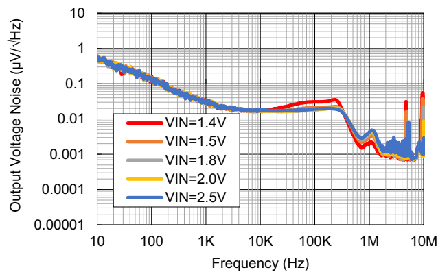
Figure 13. Output Voltage Noise for Various V_{IN} ( V_{OUT} = 0.5\text{V} , I_{OUT} = 3\text{A} )
