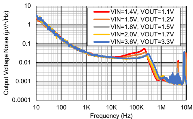
Figure 8. Output Voltage Noise for Various V_{OUT} ( V_{IN} = V_{OUT} + 0.3\text{V} , I_{OUT} = 3\text{A} , C_{NR/SS} = 0.1\mu\text{F} )
