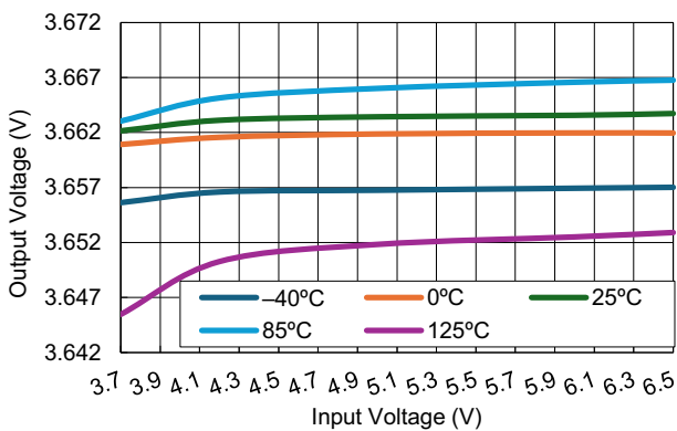
Figure 35. Line Regulation vs Input Voltage ( V_{OUT} = 3.6\text{V} , I_{OUT} = 5\text{mA} )
