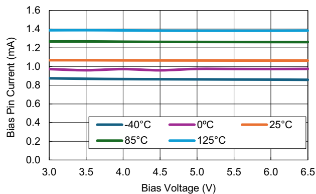
Figure 38. V_{BIAS} Quiescent Current vs Bias Voltage for Various Temperatures ( V_{IN} = 1.1\text{V} )
