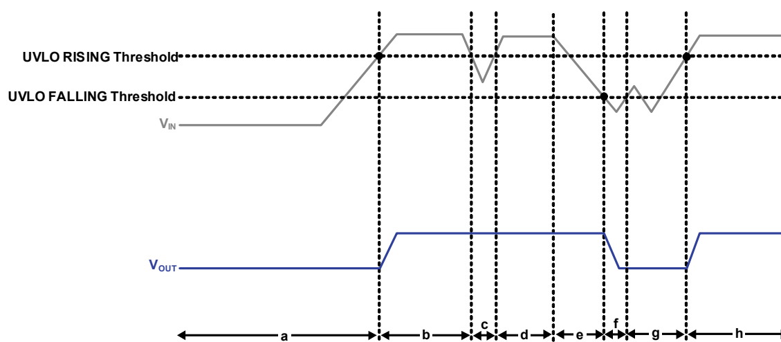
Figure 43. UVLO Operation
