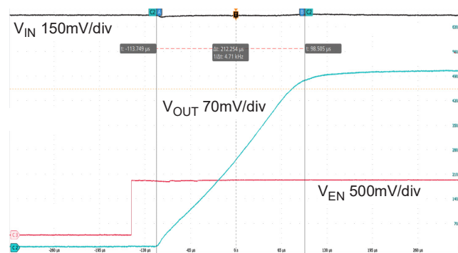
Figure 17. Start-Up ( V_{IN} = 1.4\text{V} , V_{OUT} = 0.5\text{V} , I_{OUT} = 0\text{A} )
