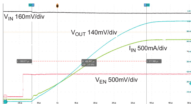
Figure 16. Start-Up ( V_{IN} = 1.4\text{V} , V_{OUT} = 1.1\text{V} , I_{OUT} = 3\text{A} (Resistive Load))
