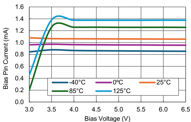
Figure 39. V_{BIAS} Quiescent Current vs Bias Voltage for Various Temperatures ( V_{IN} = 3\text{V} )
