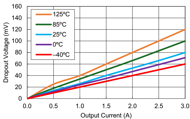
Figure 25. Dropout Voltage vs Output Current ( V_{OUT} = 3.3\text{V} )
