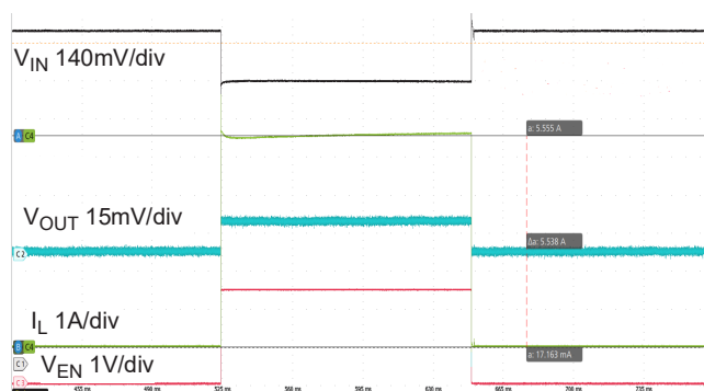
Figure 18. Start-Up with Short ( V_{IN} = 1.1\text{V} , V_{BIAS} = 5\text{V} , V_{OUT} = 0.5\text{V} )
