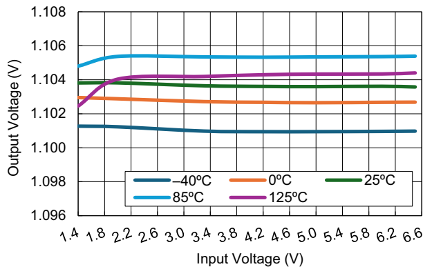
Figure 33. Line Regulation vs Input Voltage ( V_{OUT} = 1.1\text{V} , I_{OUT} = 5\text{mA} )
