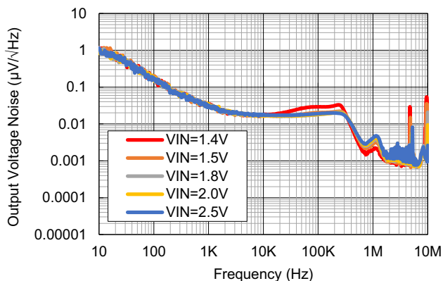
Figure 12. Output Voltage Noise for Various V_{IN} ( V_{OUT} = 0.5\text{V} , I_{OUT} = 3\text{A} , C_{NR/SS} = 0.1\mu\text{F} )
