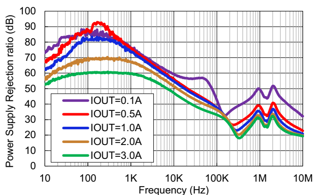
Figure 6. PSRR vs Frequency for Various I_{OUT} ( V_{IN} = 3.7\text{V} , V_{OUT} = 0.8\text{V} , C_{NR/SS} = 0.1\mu\text{F} )
