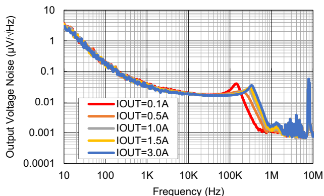
Figure 14. Output Voltage Noise for Various I_{OUT} ( V_{IN} = 3.8\text{V} , V_{OUT} = 3.3\text{V} , C_{NR/SS} = 0.1\mu\text{F} )
