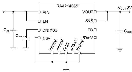
Figure 51. Internal FB Resistor Configuration for 3V ( V_{OUT} = 0.5V_{REF} + 1.6V + 800mV + 100mV )
