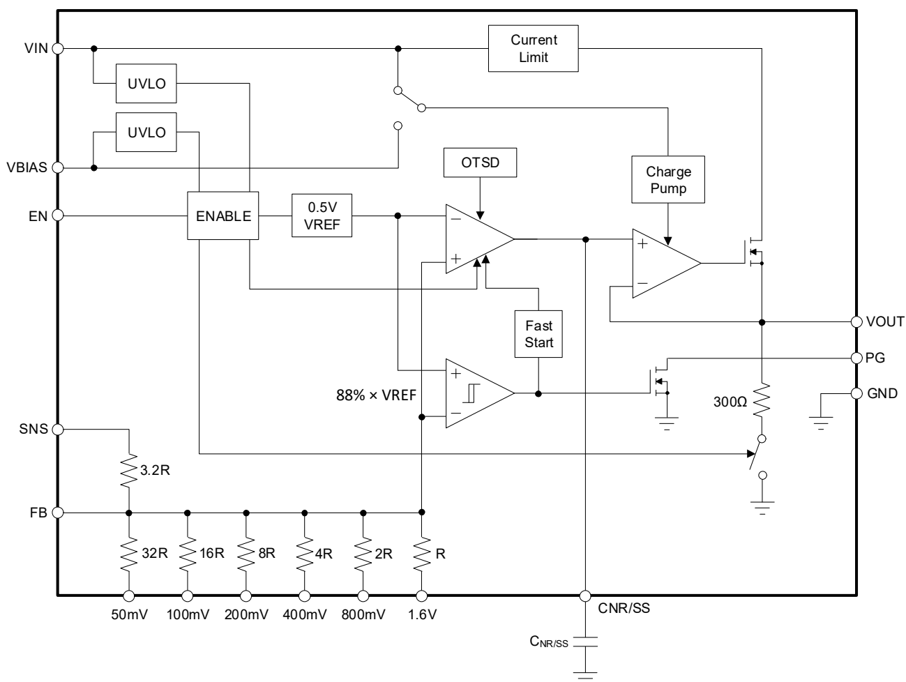
Figure 2. Block Diagram
