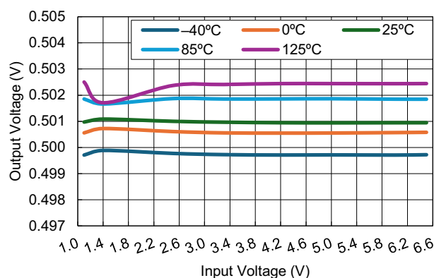
Figure 32. Line Regulation vs Input Voltage ( V_{OUT} = 0.5\text{V} , I_{OUT} = 5\text{mA} )
