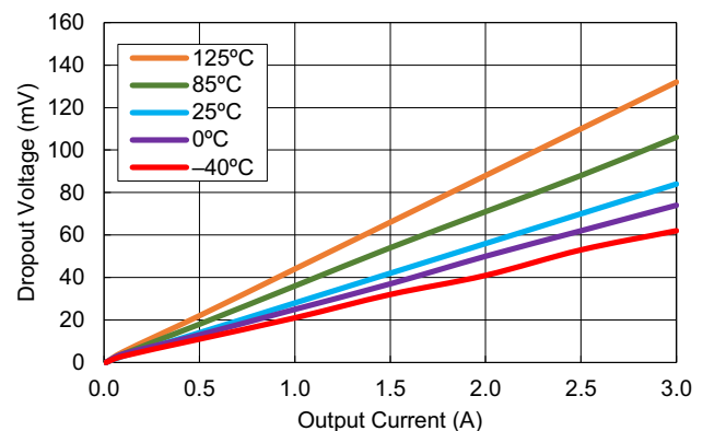
Figure 26. Dropout Voltage vs Output Current ( V_{OUT} = 5.1\text{V} )
