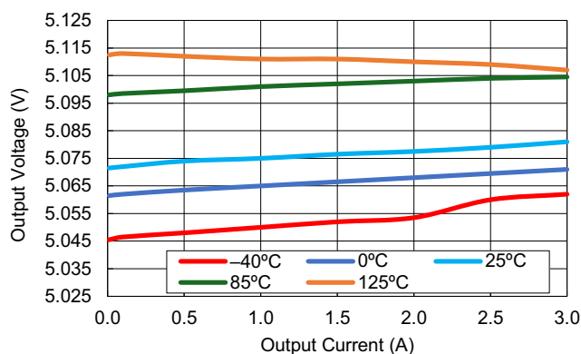
Figure 30. Load Regulation vs Output Current ( V_{OUT} = 5.1\text{V} )
