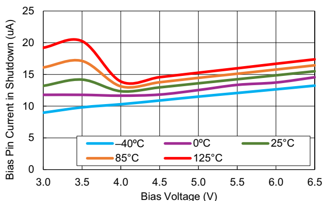
Figure 41. Shutdown Current vs Bias Voltage for Various Temperatures ( V_{IN} = 1.1\text{V} )
