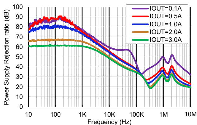
Figure 7. PSRR vs Frequency for Various I_{OUT} ( V_{IN} = 3.7\text{V} , V_{OUT} = 3.3\text{V} )
