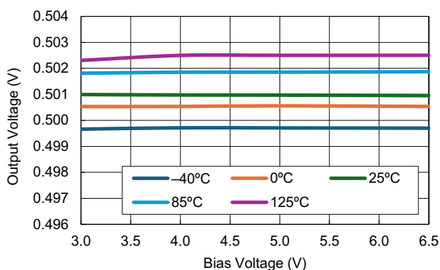
Figure 31. Line Regulation vs Bias Voltage ( V_{IN} = 1.1\text{V} , I_{OUT} = 5\text{mA} )
