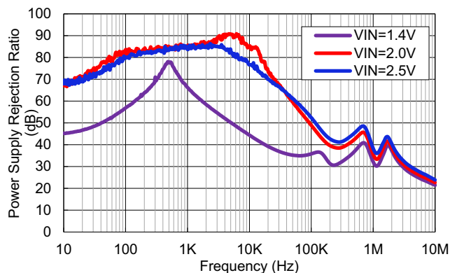
Figure 4. PSRR vs Frequency for Various V_{IN} ( I_{OUT} = 1\text{A} , C_{NR/SS} = 0.1\mu\text{F} )
