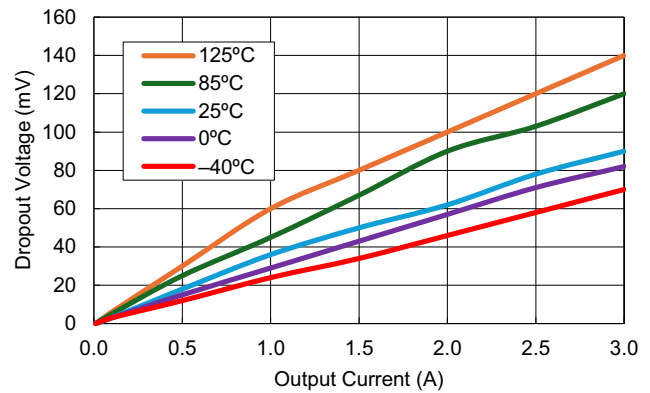
Figure 24. Dropout Voltage vs Output Current ( V_{OUT} = 1.4\text{V} )
