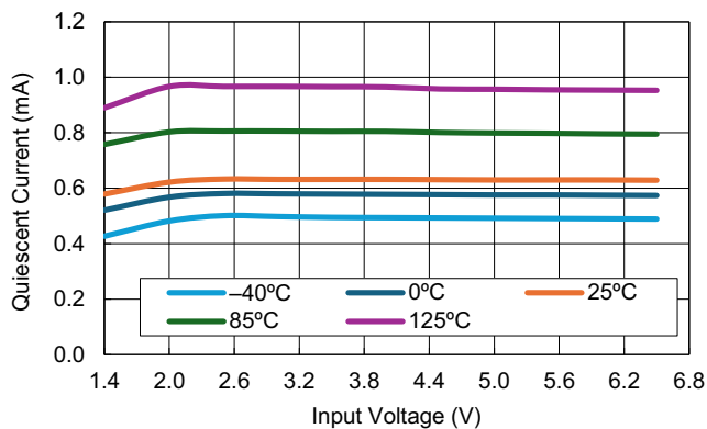
Figure 37. Quiescent Current vs Input Voltage for Various Temperatures
