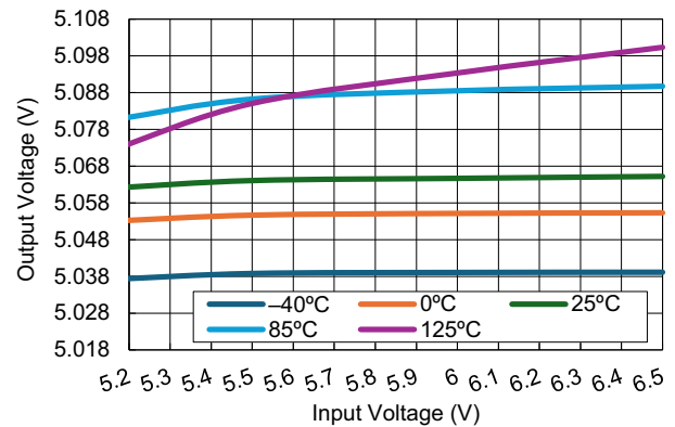
Figure 36. Line Regulation vs Input Voltage ( V_{OUT} = 5.1\text{V} , I_{OUT} = 5\text{mA} )
