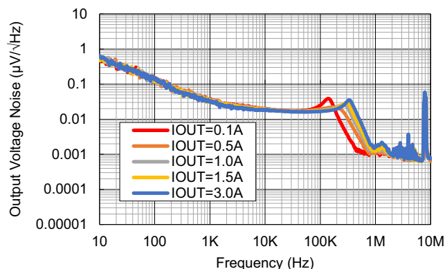
Figure 15. Output Voltage Noise for Various I_{OUT} ( V_{IN} = 3.8\text{V} , V_{OUT} = 3.3\text{V} )
