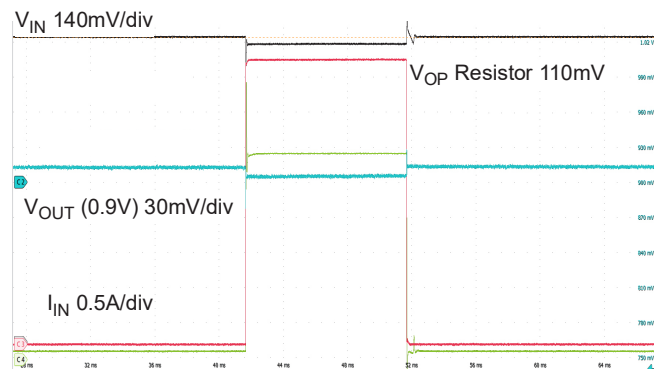
Figure 20. Load Transient Response ( V_{IN} = 1.2\text{V} , V_{BIAS} = 5\text{V} , V_{OUT} = 0.9\text{V} , \Delta I_{OUT} = 0.1\text{A} to 2.9\text{A} at 1\text{A}/\mu\text{s} )
