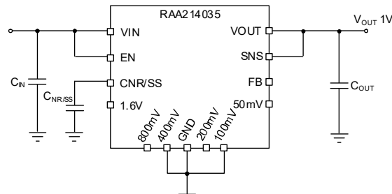
Figure 45. Internal FB Resistor Configuration for 1V ( V_{OUT} = 0.5V_{REF} + 400mV + 100mV )
