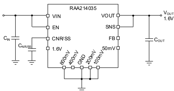
Figure 48. Internal FB Resistor Configuration for 1.6V ( V_{OUT} = 0.5V_{REF} + 800mV + 200mV + 100mV )
