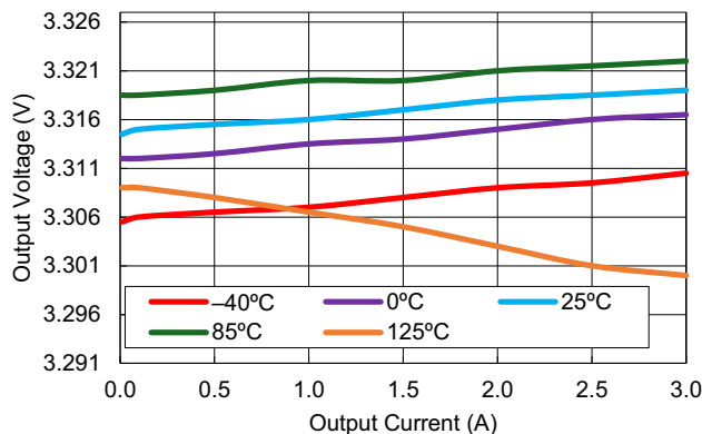
Figure 29. Load Regulation vs Output Current ( V_{OUT} = 3.3\text{V} )
