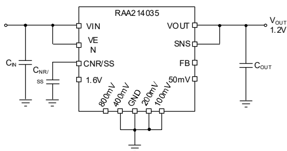
Figure 46. Internal FB Resistor Configuration for 1.2V ( V_{OUT} = 0.5V_{REF} + 400mV + 200mV + 100mV )
