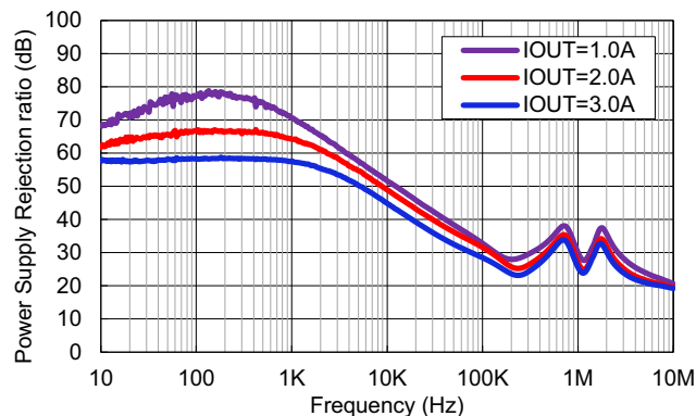
Figure 5. PSRR vs Frequency for Various I_{OUT} ( V_{IN} = 1.1\text{V} , V_{OUT} = 0.8\text{V} , V_{BIAS} = 5\text{V} , C_{NR/SS} = 0.1\mu\text{F} )
