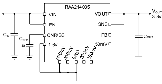
Figure 52. Internal FB Resistor Configuration for 3.3V ( V_{OUT} = 0.5V_{REF} + 1.6V + 800mV + 400mV )
