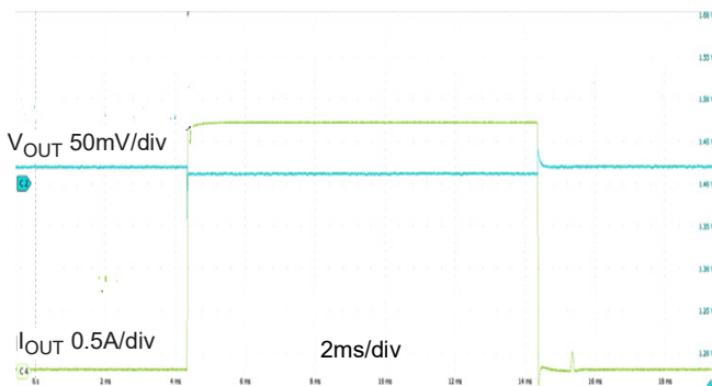
Figure 19. Load Transient Response ( V_{IN} = 1.8\text{V} , V_{OUT} = 1.4\text{V} , \Delta I_{OUT} = 0\text{A} to 3\text{A} at 1\text{A}/\mu\text{s} , C_{NR/SS} = 0.1\mu\text{F} )
