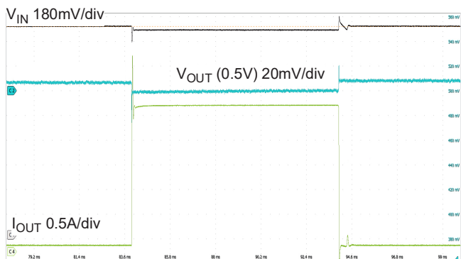
Figure 21. Load Transient Response for ( V_{IN} = 1.4\text{V} , V_{OUT} = 0.5\text{V} , \Delta I_{OUT} = 0.1\text{mA} to 3\text{A} at 1\text{A}/\mu\text{s} )
