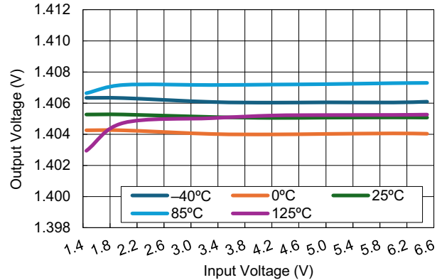
Figure 34. Line Regulation vs Input Voltage ( V_{OUT} = 1.4\text{V} , I_{OUT} = 5\text{mA} )
