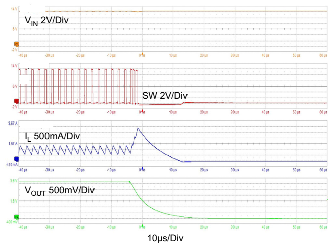
Figure 32. I_{OUT} = 1\text{A} to Short-Circuit
