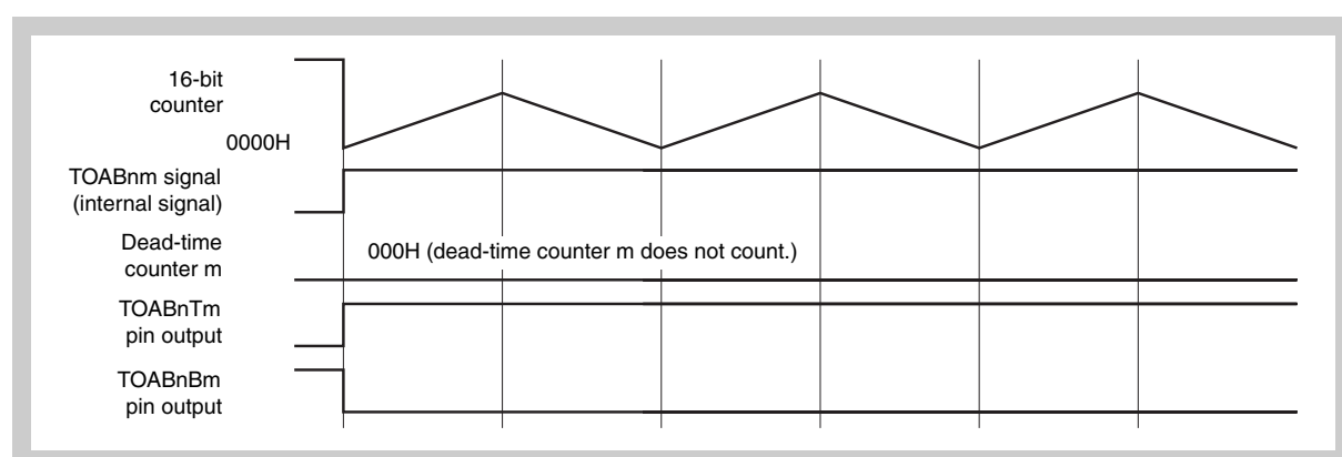
Figure 22-16 PWM Output Waveform with Dead Time (2) 100% output (TABnCCRM register = 0000H, TABnCCR0 register = M, TABnDTC register = a)
