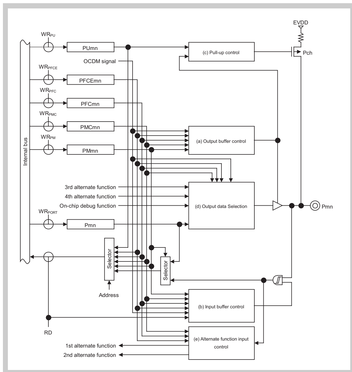
Figure 2-36 Port type F11000-U block diagram
