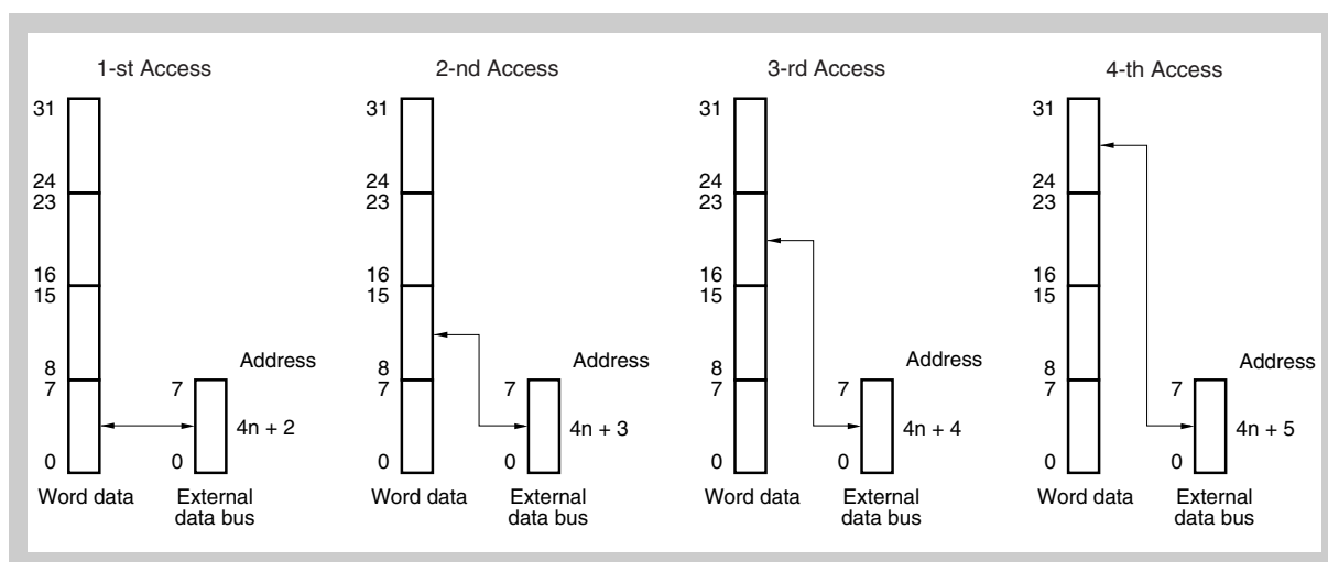
Figure 9-17 Access to address 4n + 2
