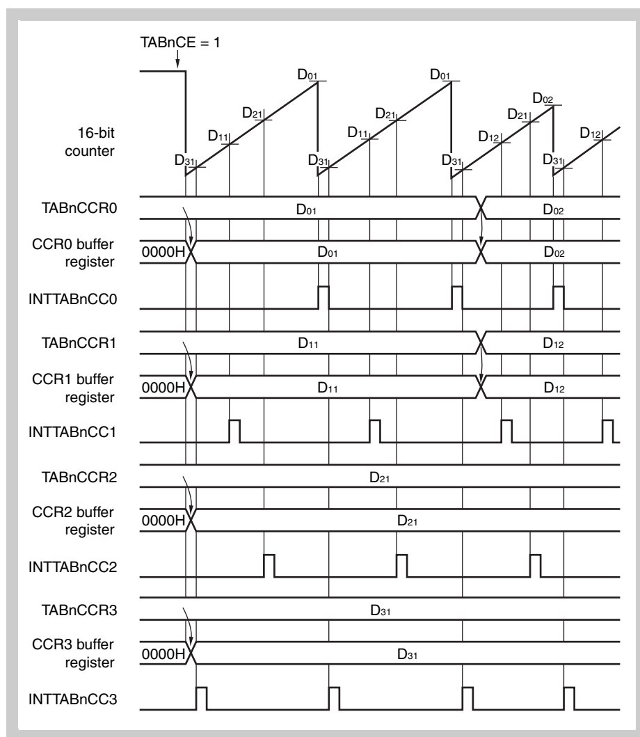
Figure 12-3 Timing chart of anytime write
