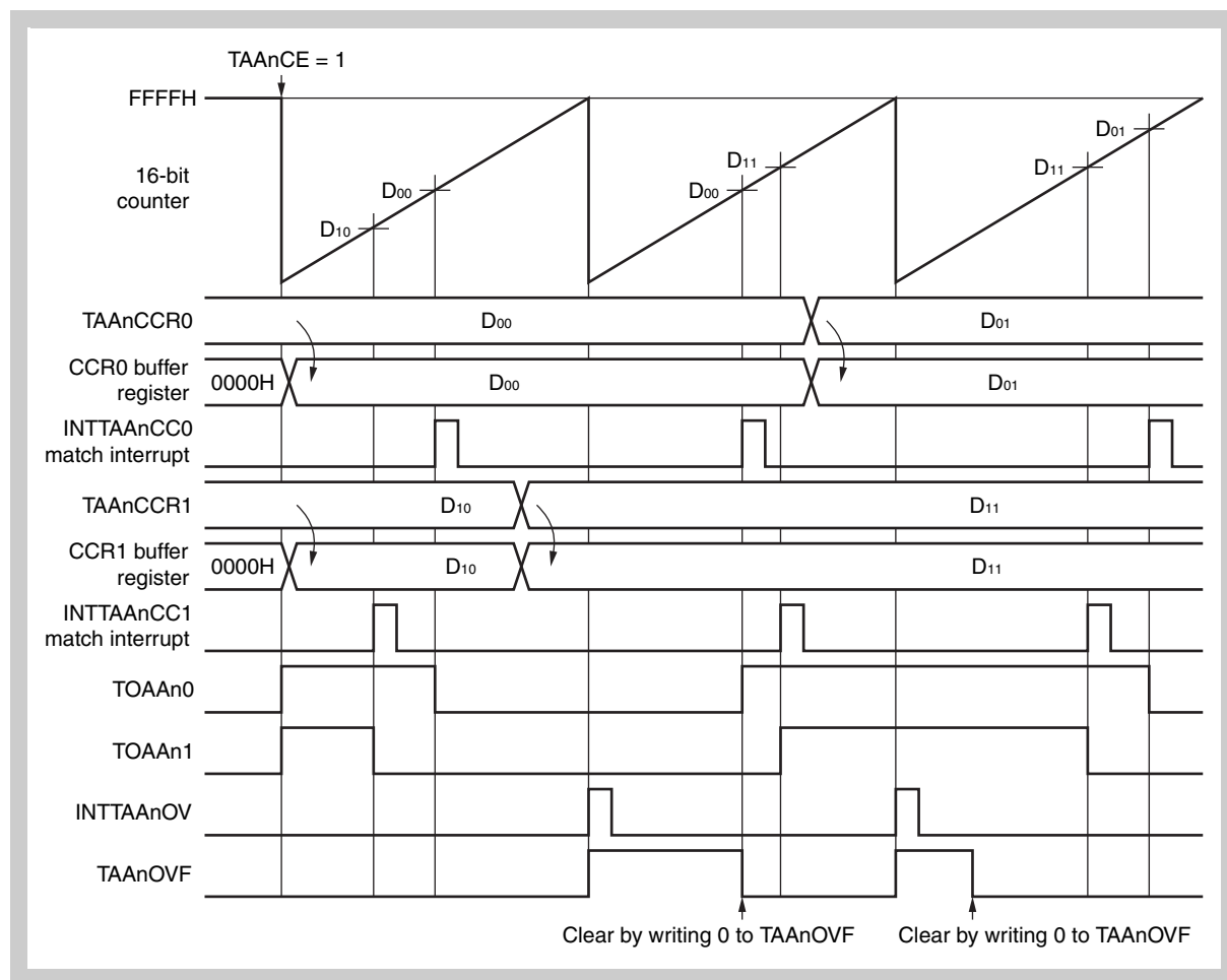
Figure 11-26 Basic Operation Timing in Free-Running Mode (TAA n CCS1 = 0, TAA n CCS0 = 0) (TAA n OEm = 1, TAA n OEL = 1, TAA n OL0 = 0, TAA n OL1 = 0)
