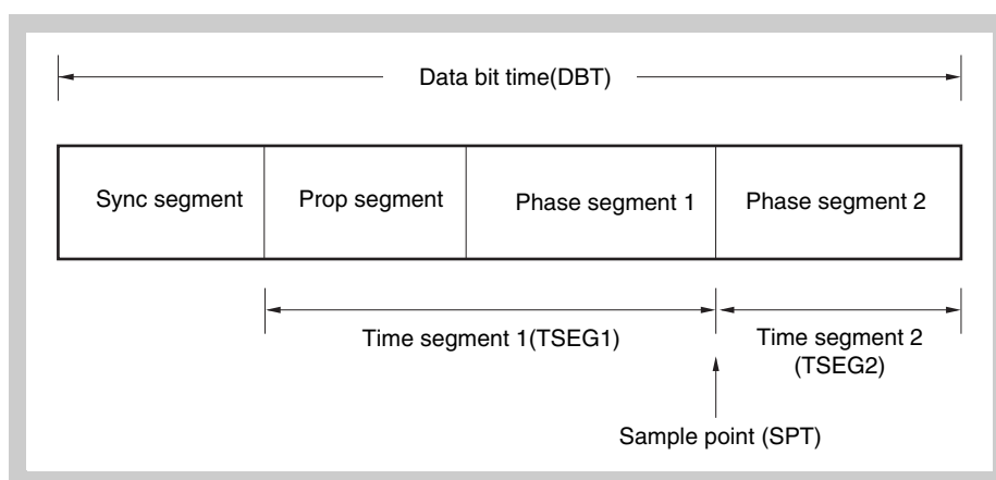
Figure 20-18 Segment setting
