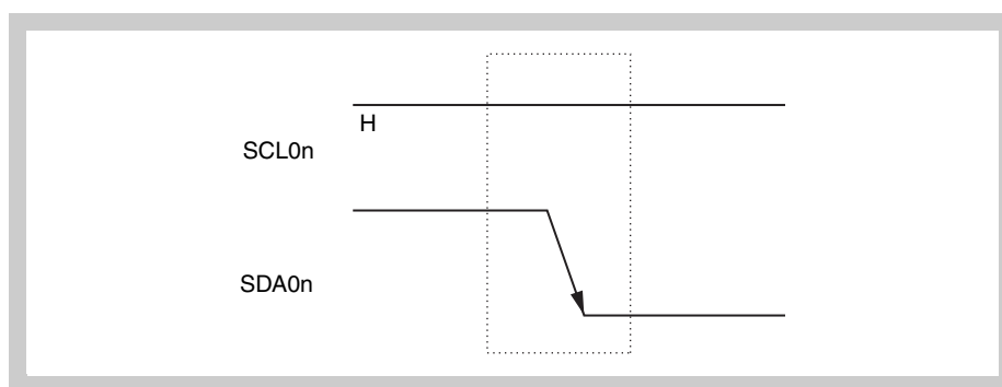
Figure 19-6 Start condition
