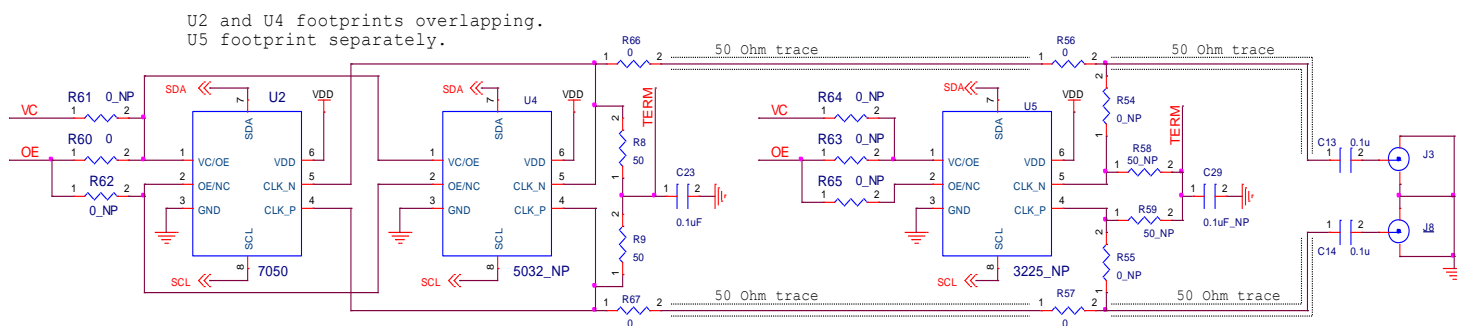
Figure 2. Output Terminations
