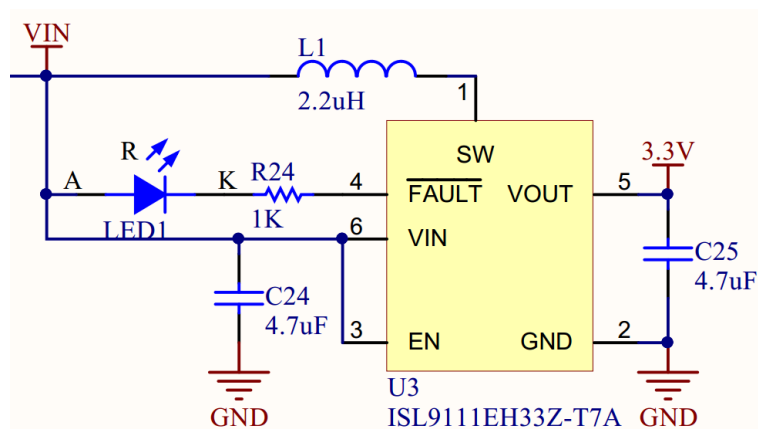
Figure 10. Boost Circuit
