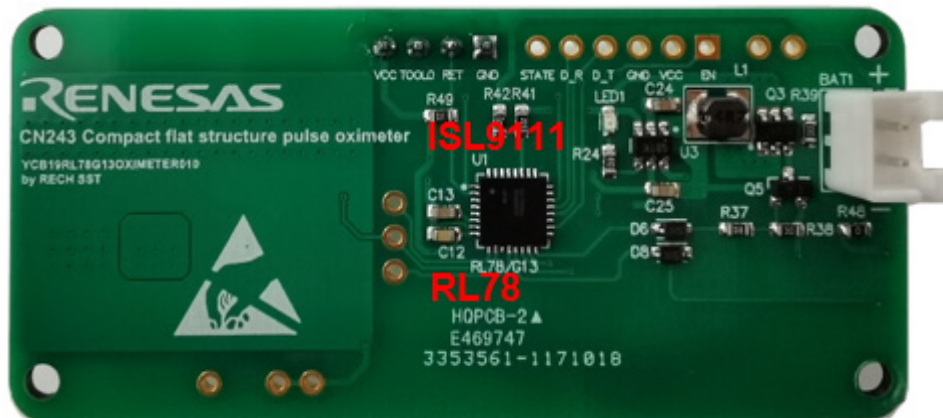
Figure 7. OB1203SD-RL-EVK (Bottom)
