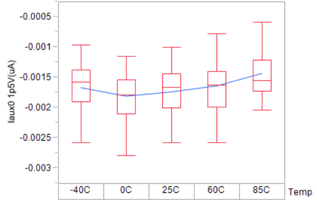
Figure 24. AUX0/xT0 Pin Input Current at 1.5V
