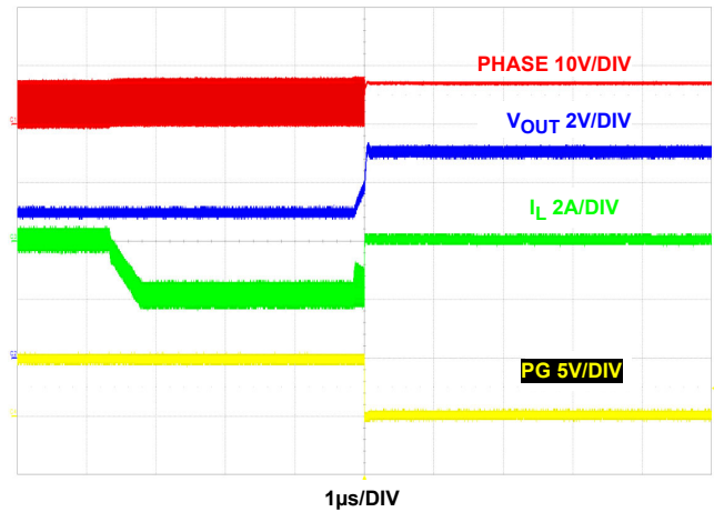
FIGURE 39. OVERVOLTAGE PROTECTION
