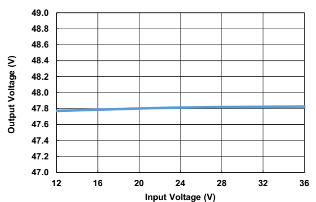
Figure 23. CCM Line Regulation at 3A Load +25°C
