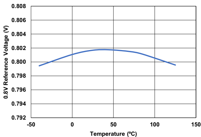
Figure 15. 0.8V Reference Voltage vs Temperature
